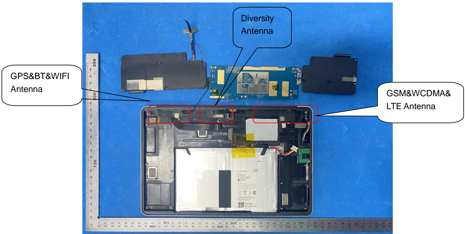
OPEN VIEW OF EUT(FIGURE 2)
