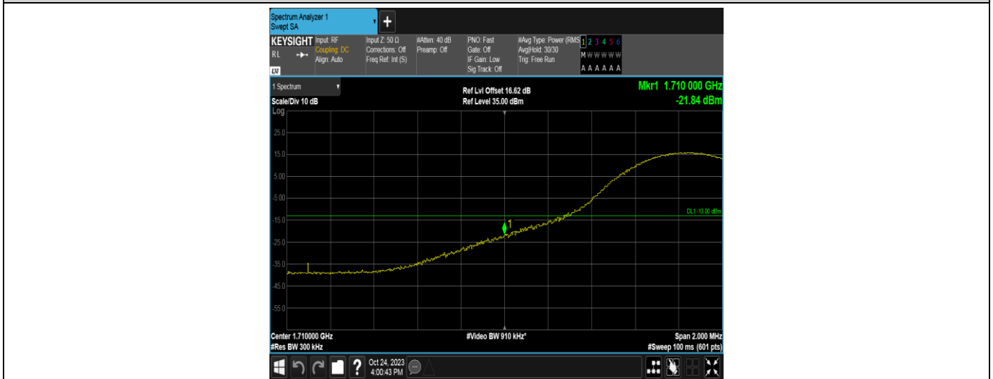
Band4-15MHz-16QAM-20025-1RB#0
