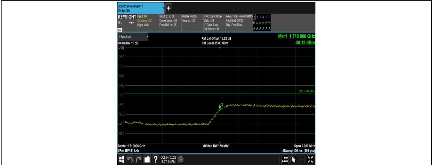
Band4-3MHz-QPSK-19965-15RB#0
