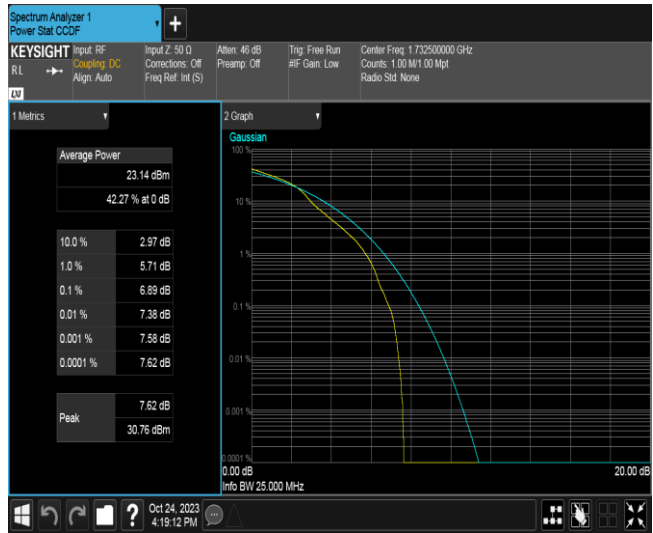
Band4-20MHz-16QAM-20175-100RB#0
