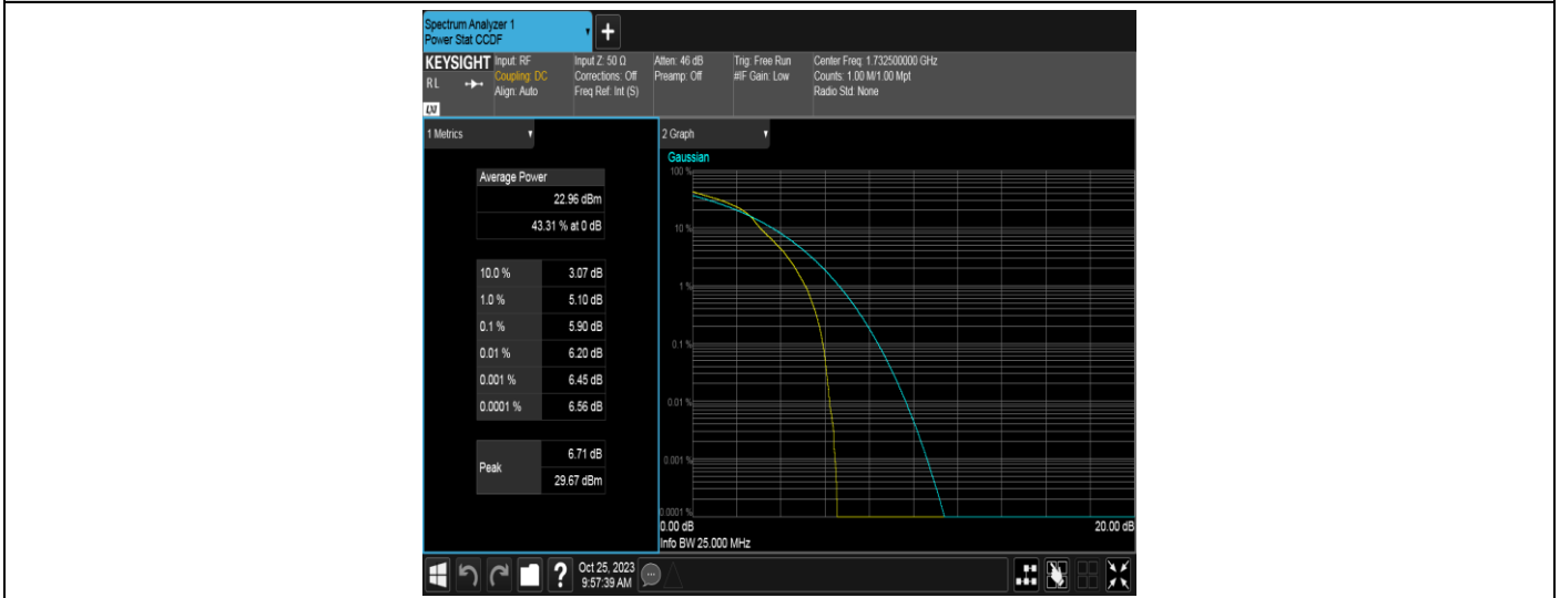
Band4-10MHz-16QAM-20175-1RB#0
