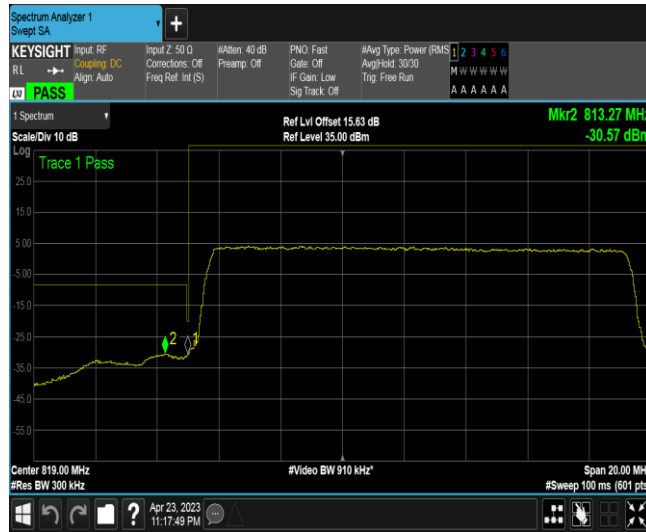
Band26-15MHz-16QAM-26765-1RB#0
