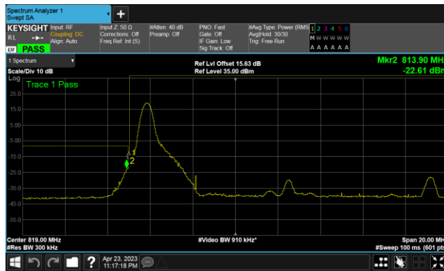
Band26-15MHz-16QAM-26765-1RB#74
