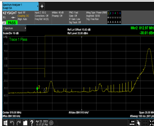
Band26-15MHz-16QAM-26765-75RB#0
