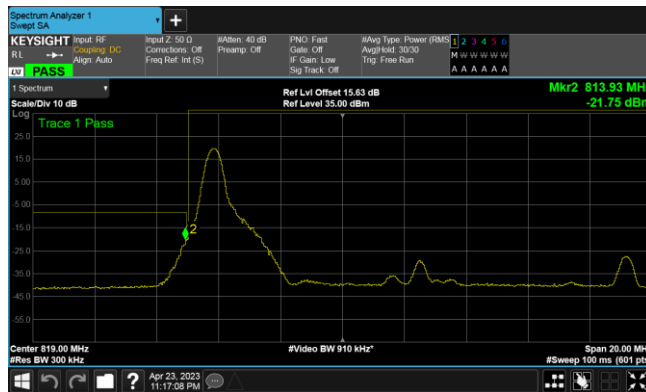
Band26-15MHz-QPSK-26765-1RB#74
