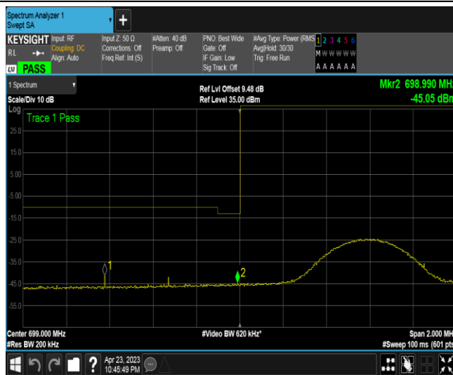
Band12-10MHz-16QAM-23060-1RB#49
