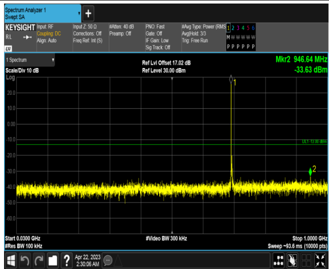
Band12-3MHz-16QAM-23025-1RB#0-Range1:30~1000MHz
