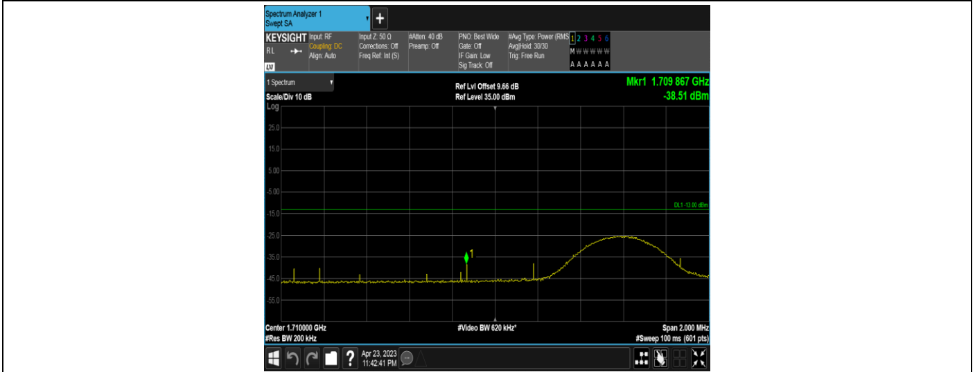
Band4-10MHz-16QAM-20000-50RB#0
