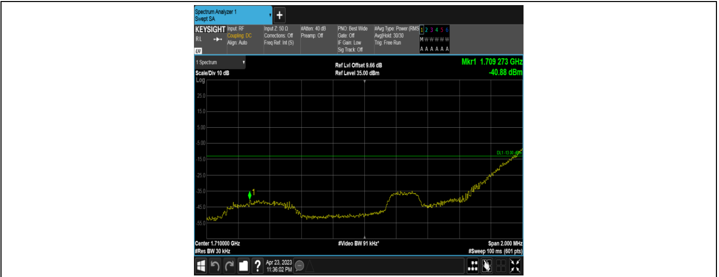
Band4-1.4MHz-16QAM-19957-6RB#0
