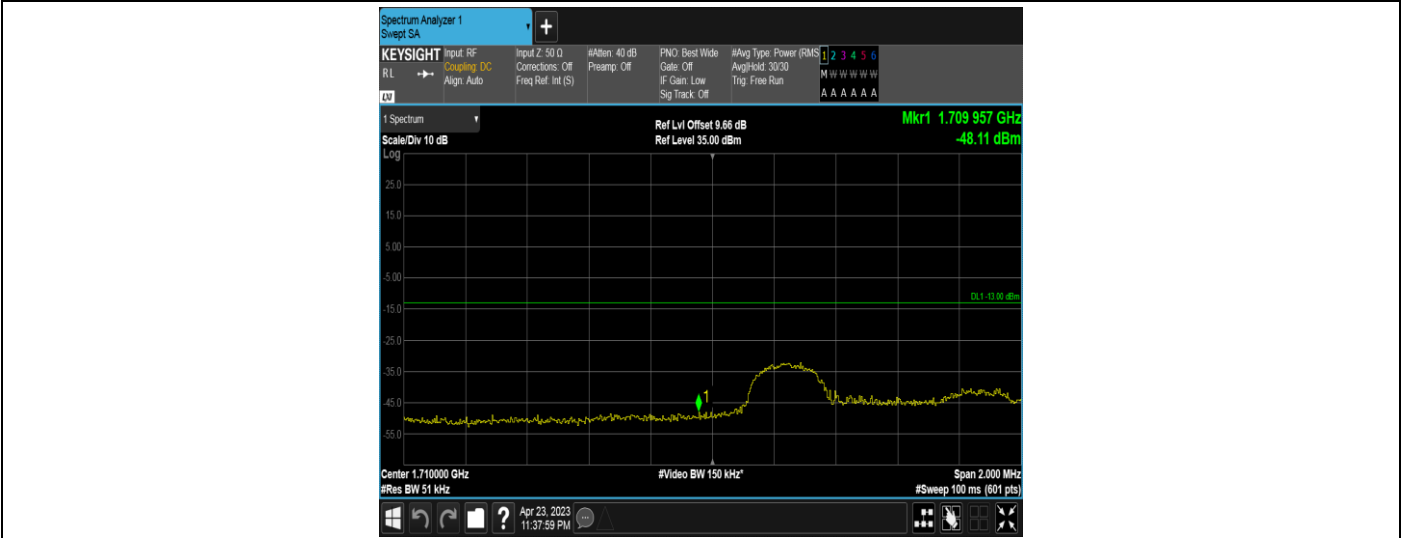
Band4-3MHz-QPSK-19965-15RB#0
