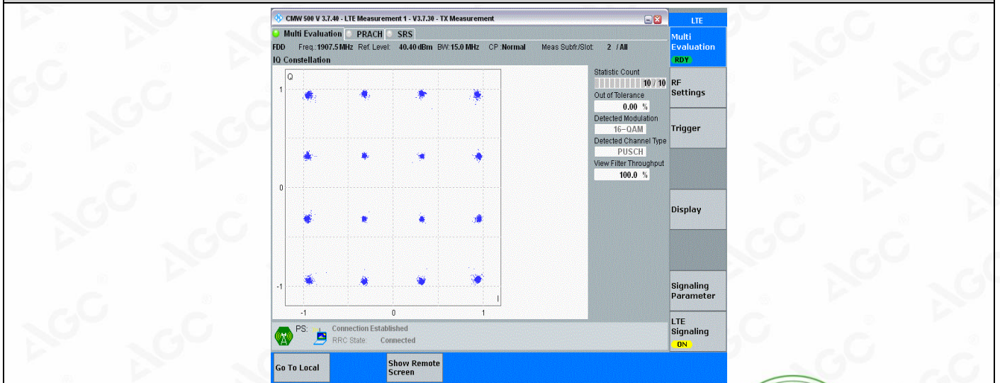
Band25-15MHz-16QAM-26615-75RB#0
