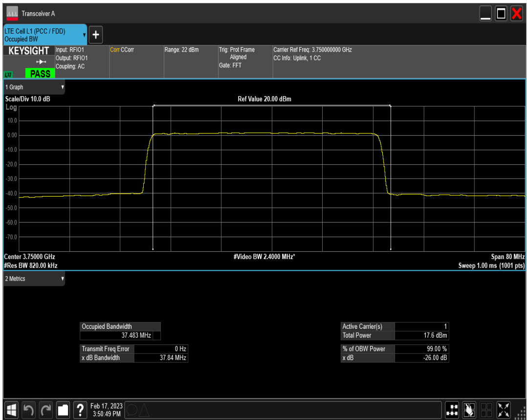
n78(3700-3800) SCS=30kHz DFT 256QAM BW=40MHz Channel=650000 RB=100@0
