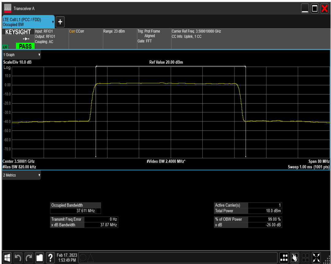
n78(3450-3550) SCS=30kHz DFT 64QAM BW=40MHz Channel=633334 RB=100@0
