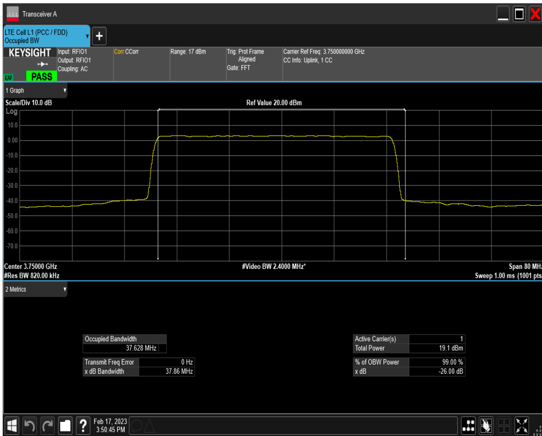
n78(3700-3800) SCS=30kHz DFT 16QAM BW=40MHz Channel=650000 RB=100@0
