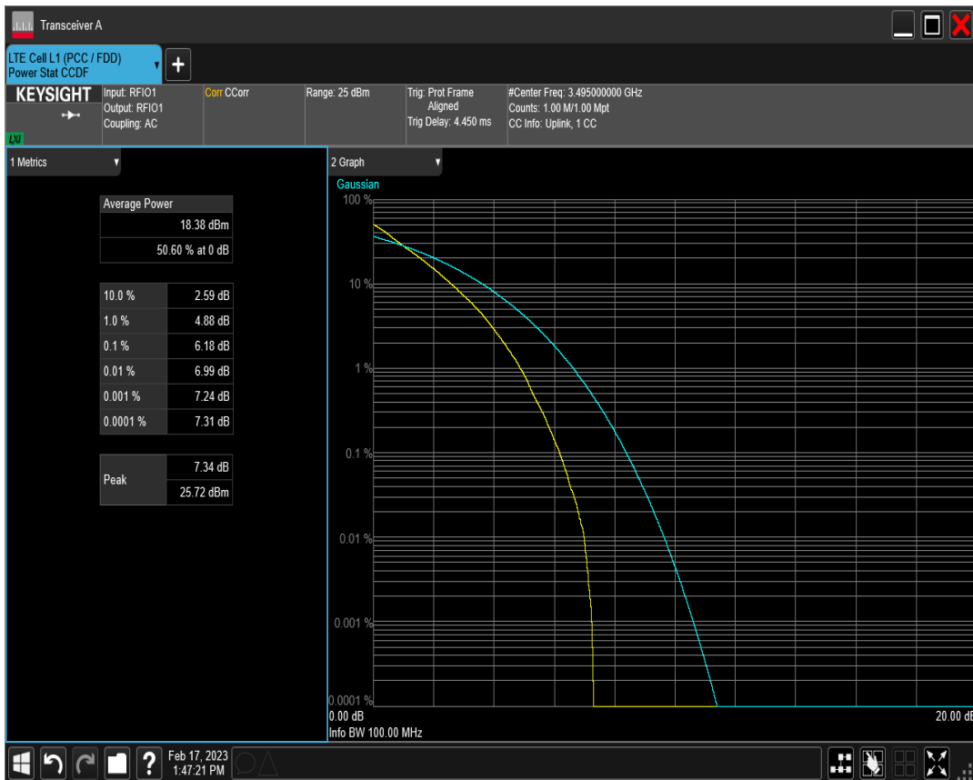
n78(3450-3550) SCS=30kHz DFT 16QAM BW=90MHz Channel=633000 RB=240@0
