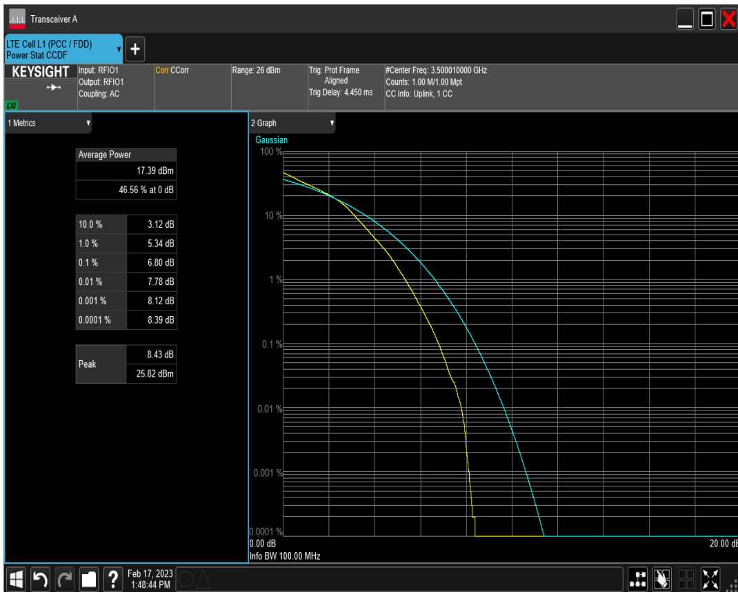
n78(3450-3550) SCS=30kHz DFT 64QAM BW=90MHz Channel=633334 RB=240 @0
