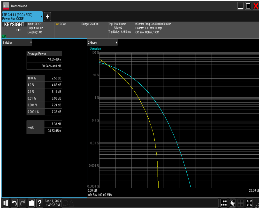
n78(3450-3550) SCS=30kHz DFT 16QAM BW=90MHz Channel=633334 RB=240 @0
