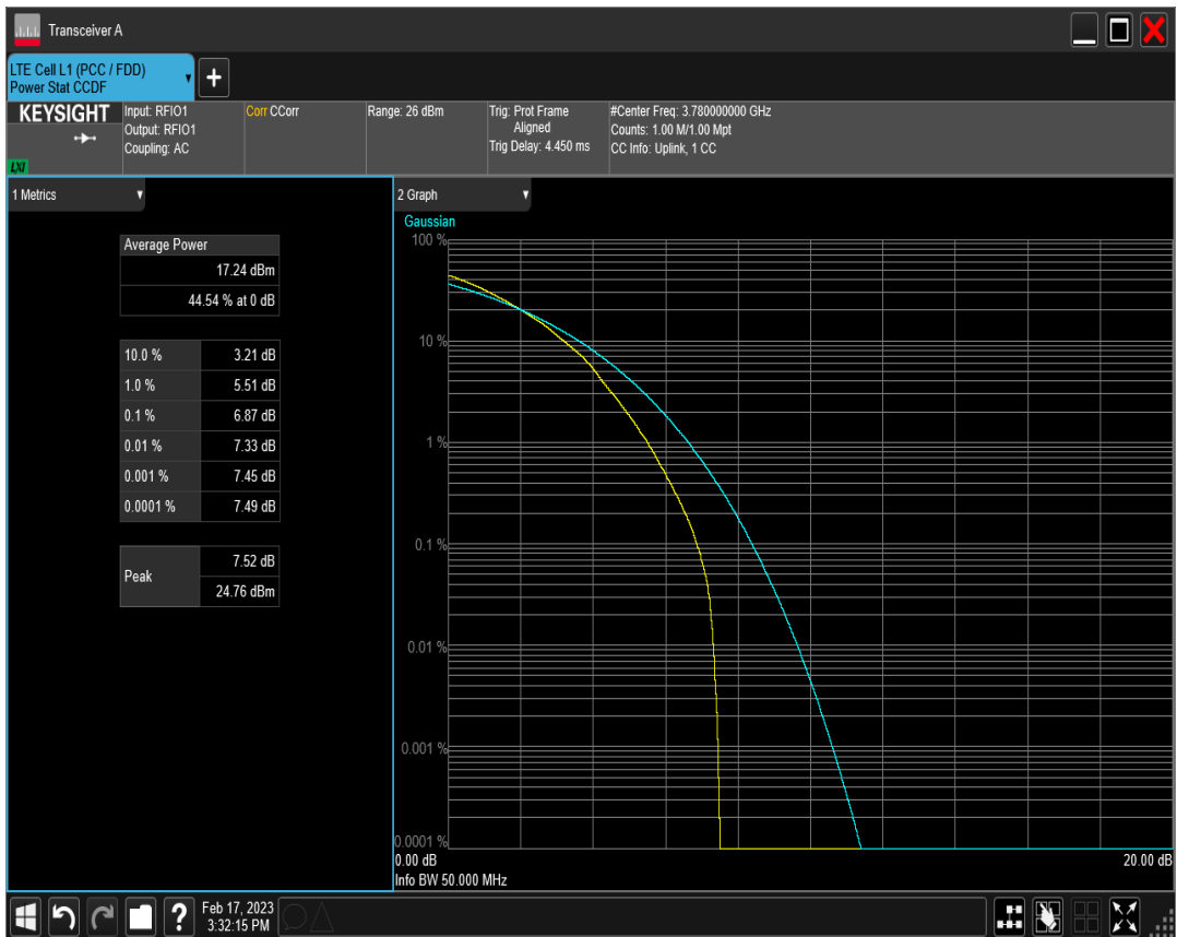
n78(3700-3800) SCS=30kHz DFT 256QAM BW=40MHz Channel=652000 RB=100@0
