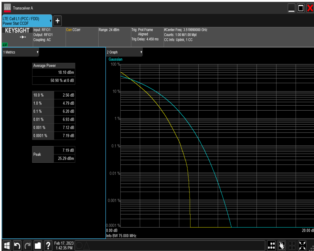
n78(3450-3550) SCS=30kHz DFT 16QAM BW=60MHz Channel=634666 RB=162@0
