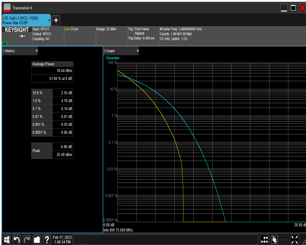
n78(3450-3550) SCS=30kHz DFT 16QAM BW=60MHz Channel=632000 RB=162@0
