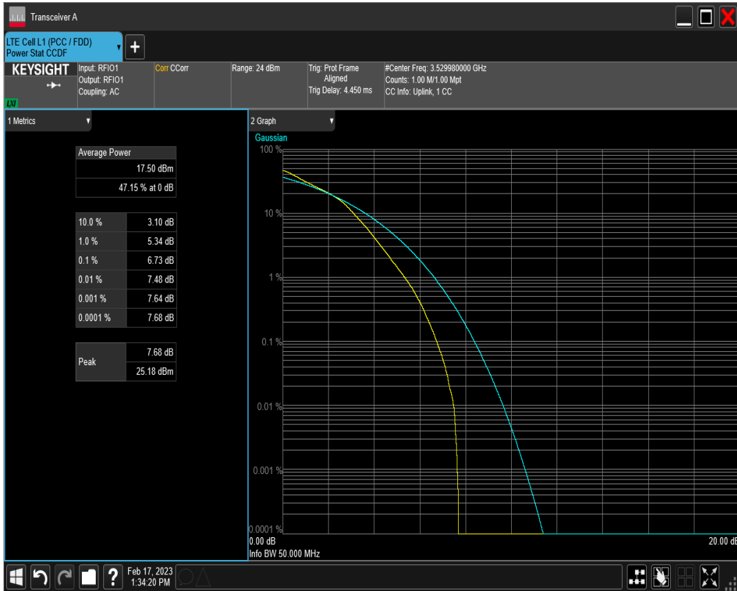
n78(3450-3550) SCS=30kHz DFT 64QAM BW=40MHz Channel=635332 RB=100@0
