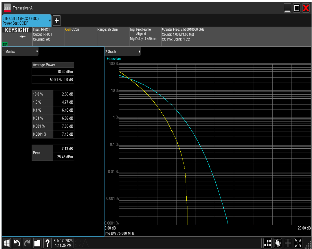
n78(3450-3550) SCS=30kHz DFT 16QAM BW=60MHz Channel=633334 RB=162@0
