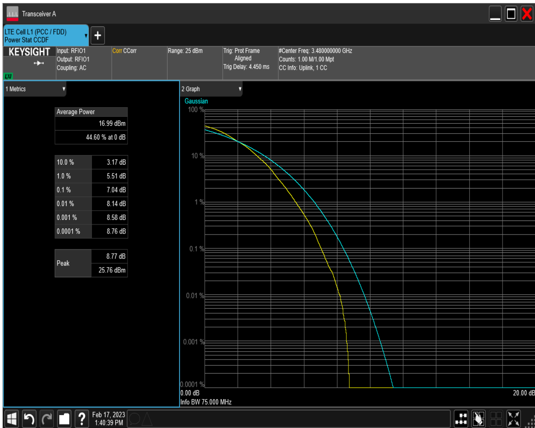
n78(3450-3550) SCS=30kHz DFT 256QAM BW=60MHz Channel=632000 RB=162@0
