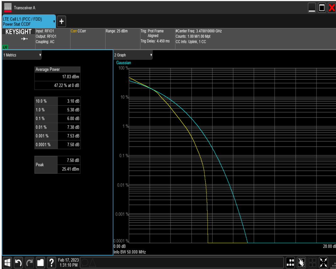
n78(3450-3550) SCS=30kHz DFT 64QAM BW=40MHz Channel=631334 RB=100@0
