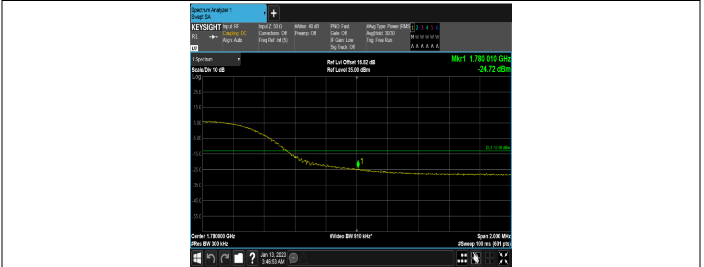
Band66-15MHz-16QAM-132047-1RB#0
