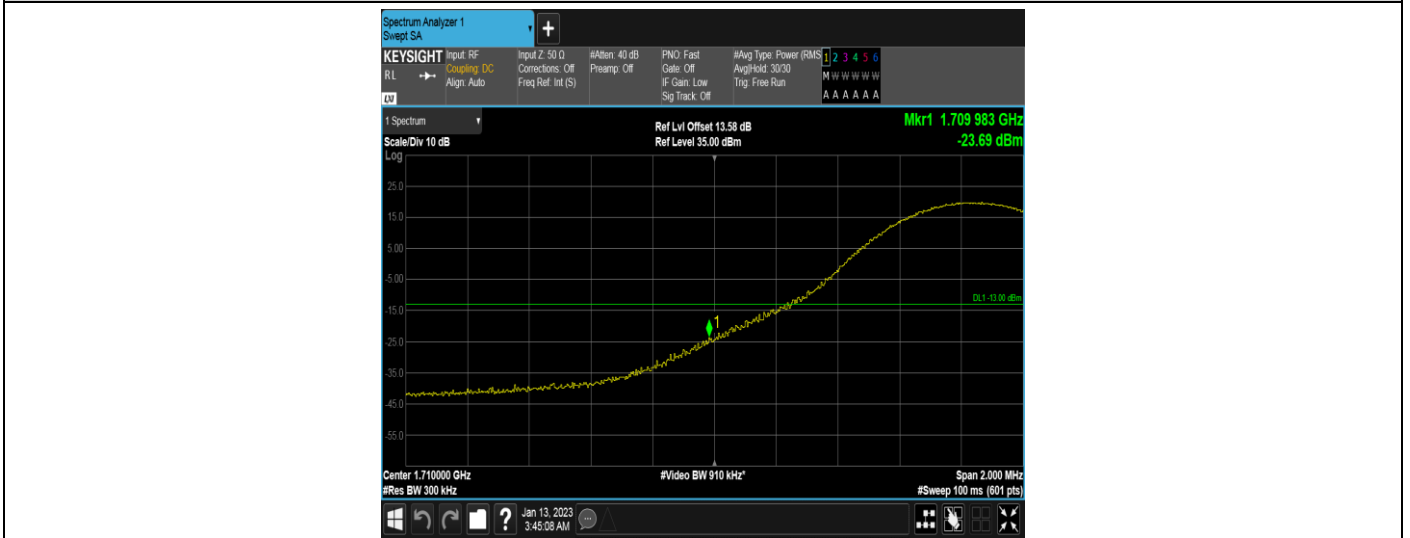
Band66-15MHz-16QAM-132047-1RB#0
