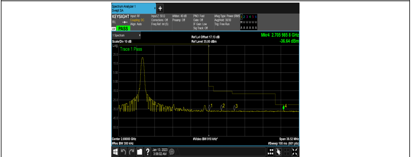
Band41-15MHz-QPSK-41515-1RB#74
