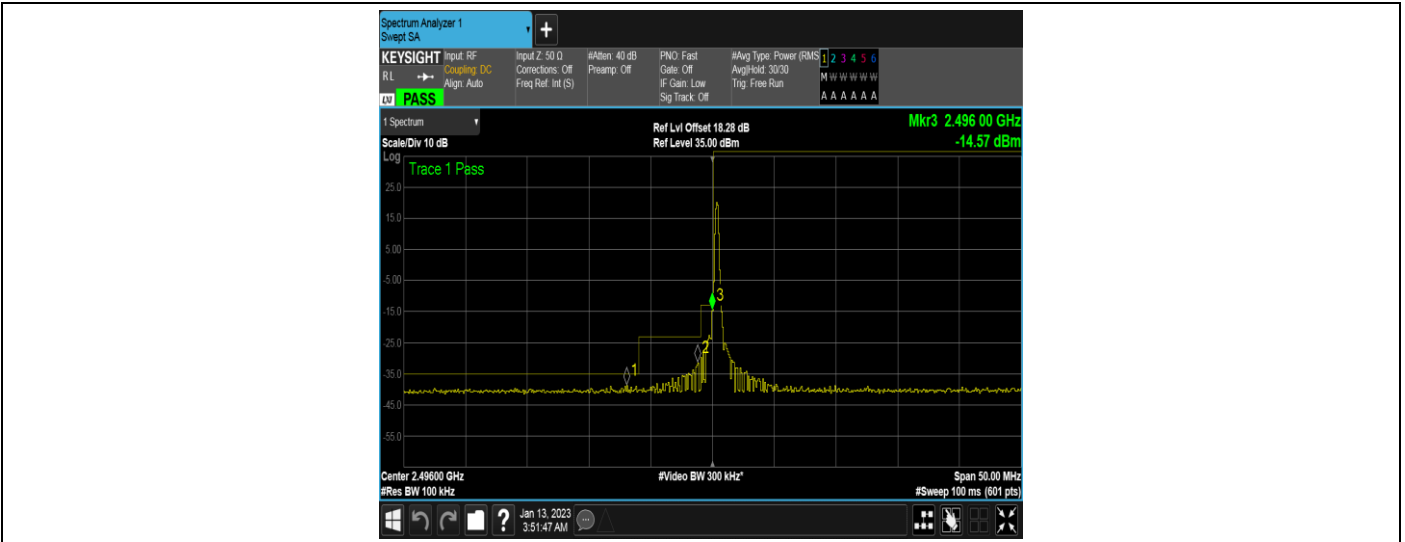
Band41-5MHz-16QAM-39675-1RB#24
