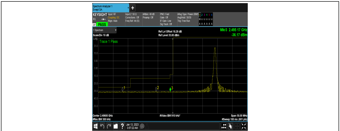
Band41-15MHz-16QAM-39725-75RB#0
