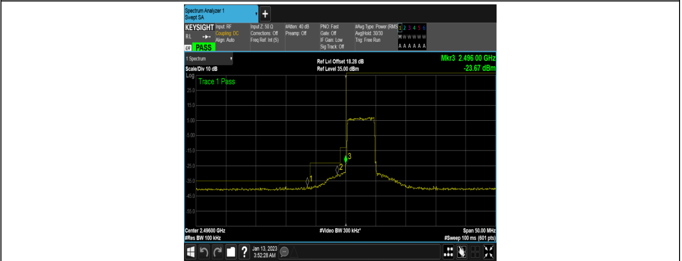
Band41-5MHz-16QAM-39675-25RB#0
