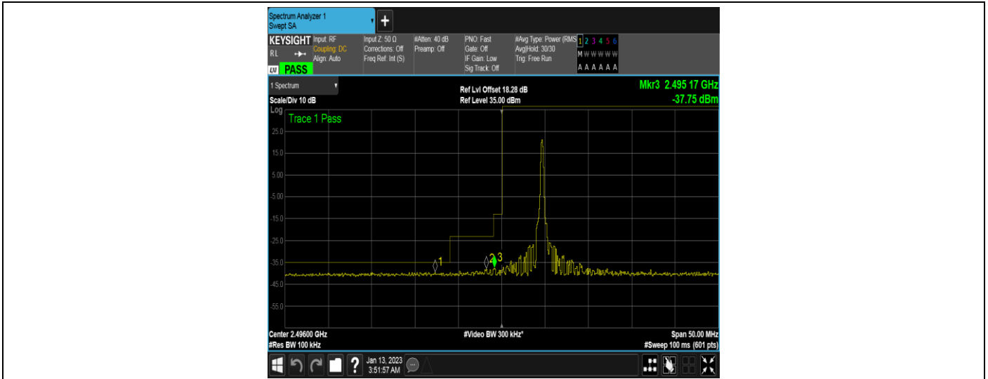
Band41-5MHz-QPSK-39675-25RB#0
