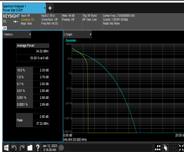
Band41-20MHz-QPSK-40620-1RB#0
