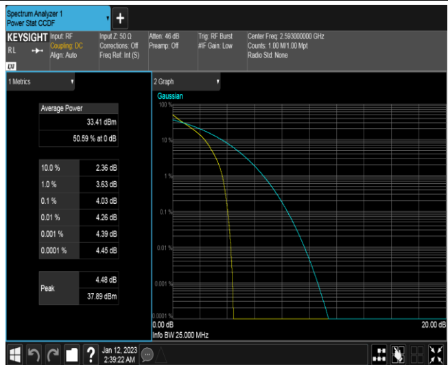
Band41-5MHz-QPSK-40620-25RB#0
