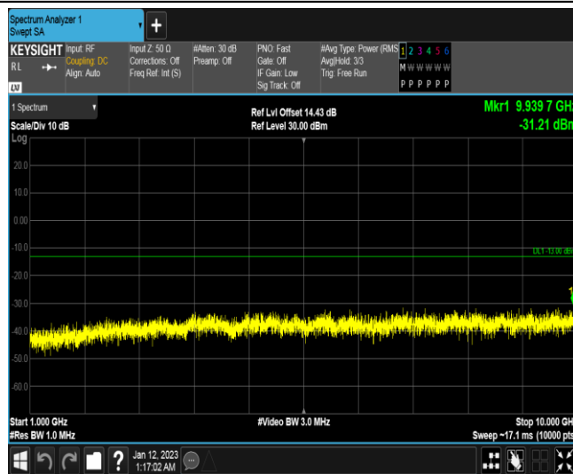
Band26-15MHz-16QAM-26765-1RB#0-Range2:1000~10000MHz
