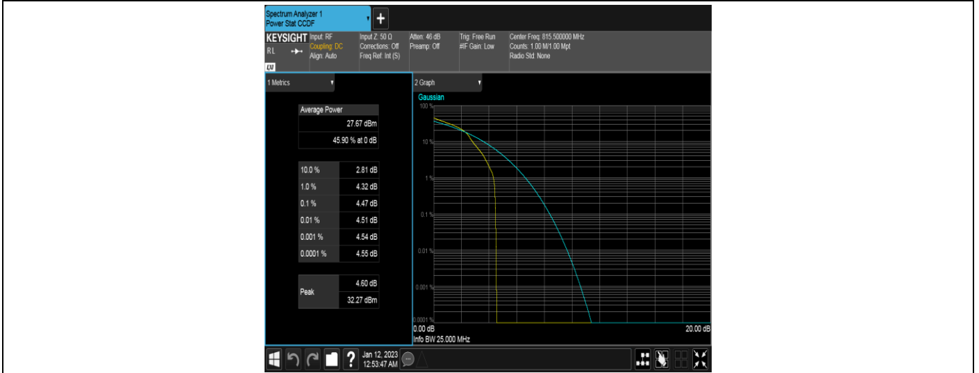
Band26-3MHz-16QAM-26705-15RB#0
