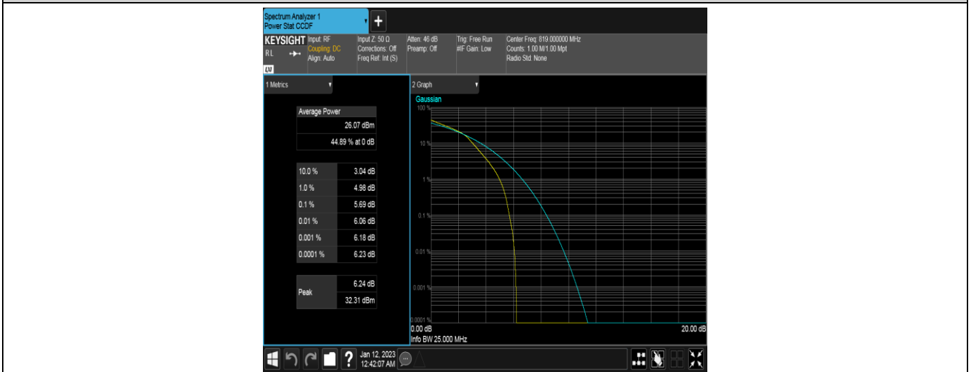
Band26-1.4MHz-16QAM-26740-6RB#0
