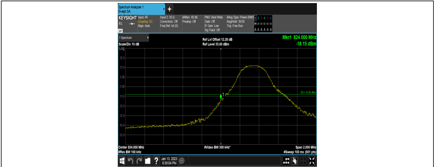
Band26-5MHz-16QAM-26815-1RB#24
