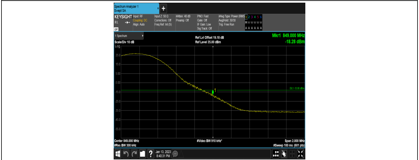
Band26-15MHz-QPSK-26965-1RB#74
