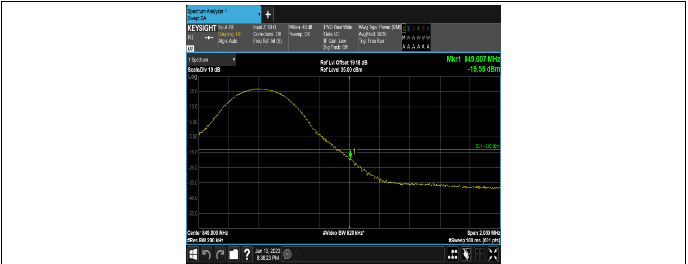
Band26-10MHz-QPSK-26990-50RB#0
