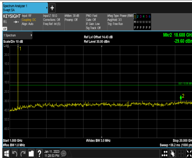
Band25-3MHz-16QAM-26055-1RB#0-Range2:1000~20000MHz
