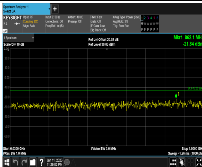
Band25-3MHz-QPSK-26365-1RB#0-Range1:30~1000MHz
