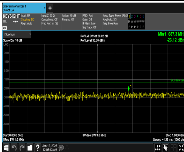
Band25-15MHz-16QAM-26115-1RB#0-Range1:30~1000MHz
