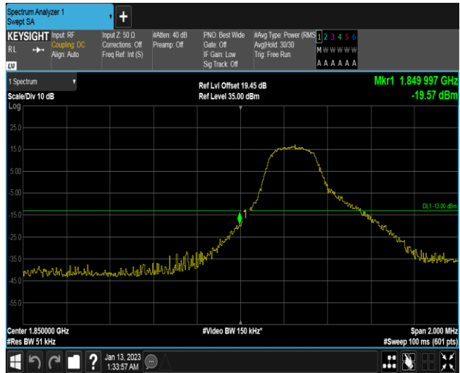
Band25-3MHz-QPSK-26055-1RB#14
