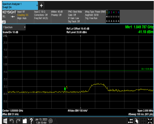
Band25-3MHz-QPSK-26055-15RB#0
