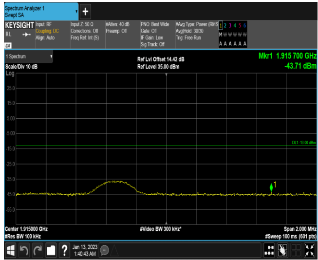
Band25-5MHz-QPSK-26665-1RB#24
