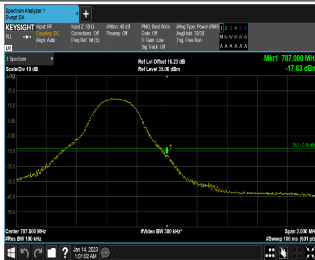
Band13-5MHz-16QAM-23255-1RB#24
