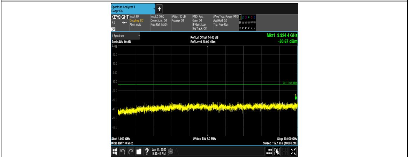
Band12-1.4MHz-QPSK-23095-1RB#0-Range2:1000~10000MHz
