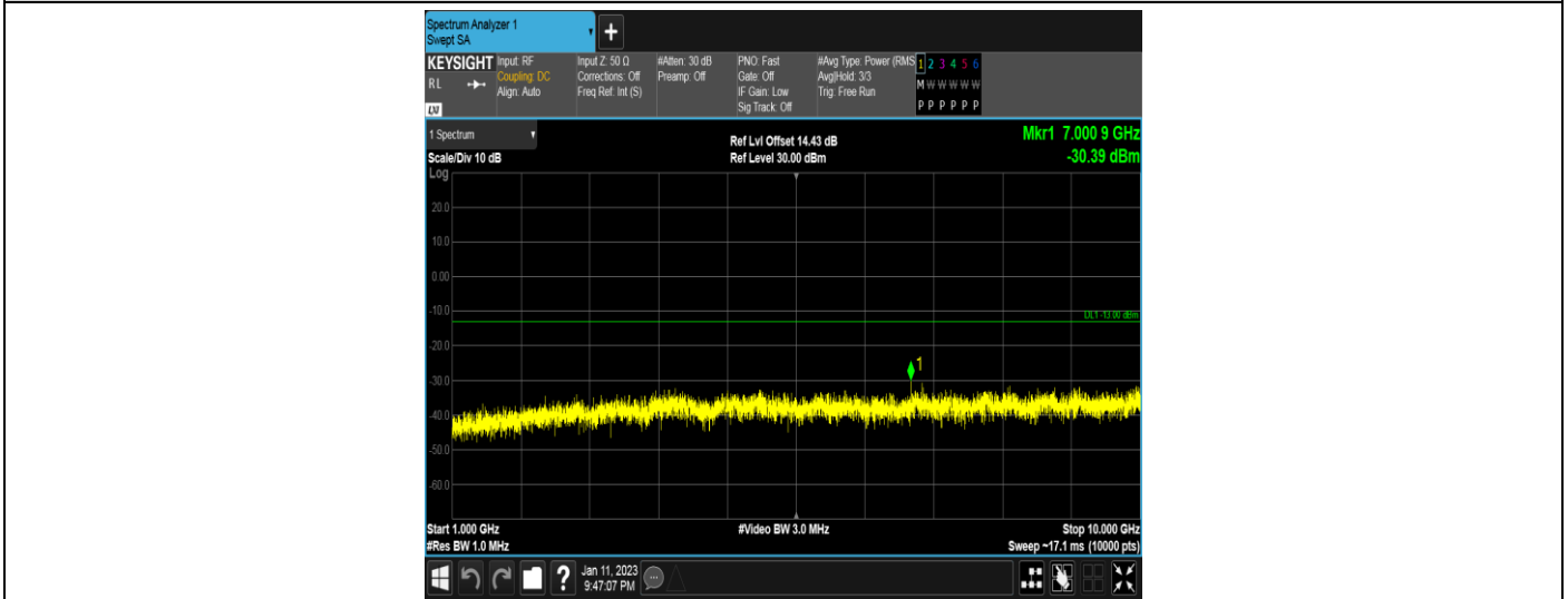
Band12-3MHz-QPSK-23025-1RB#0-Range2:1000~10000MHz
