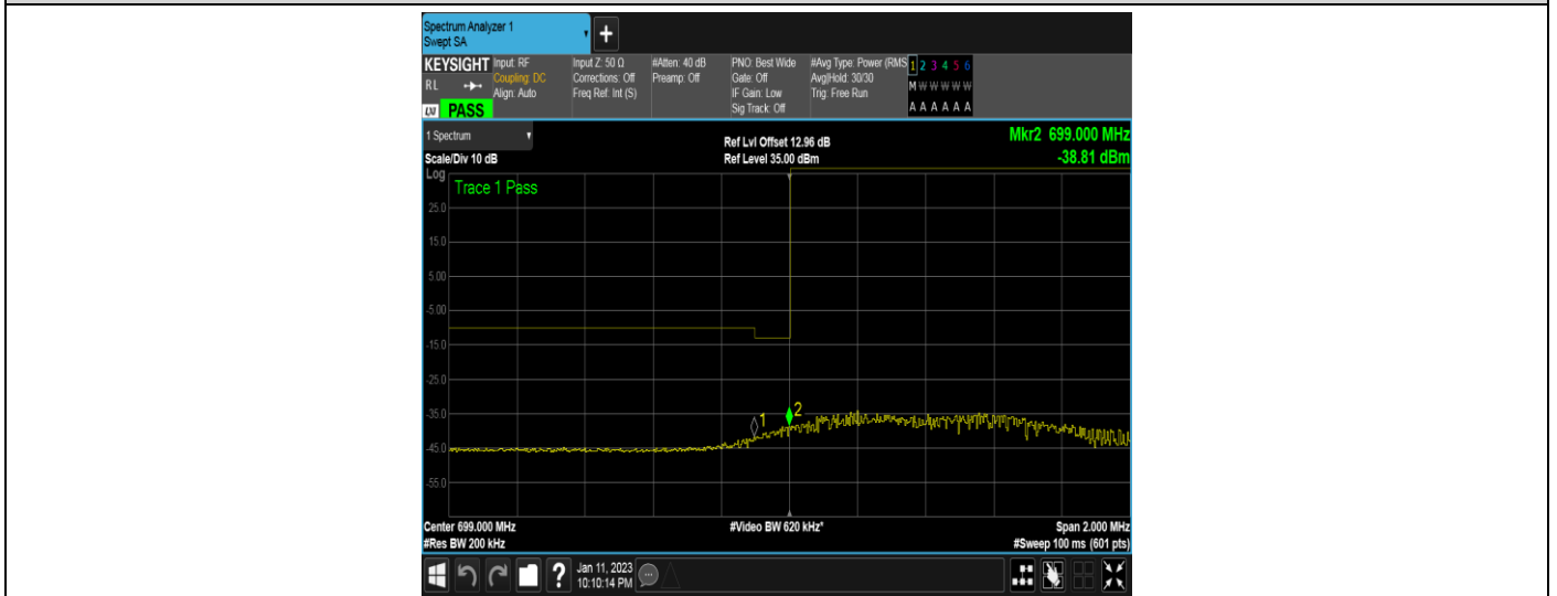
Band12-10MHz-16QAM-23060-1RB#49
