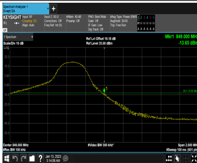
Band5-5MHz-QPSK-20625-1RB#24
