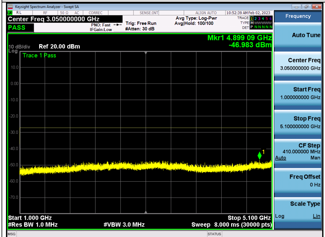
Test_Graph_802.11ax80_ANT1_5290_MCS0_Frequency Band 2
