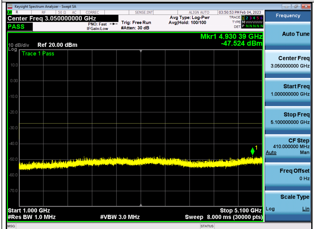
Test_Graph_802.11ax80_ANT2_5290_MCS0_Frequency Band 2
