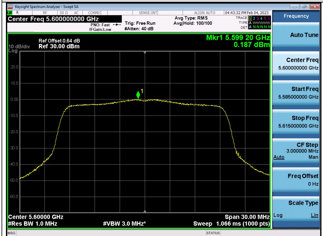
Test_Graph_802.11ax20_ANT2_5600_MCS0_PSD
