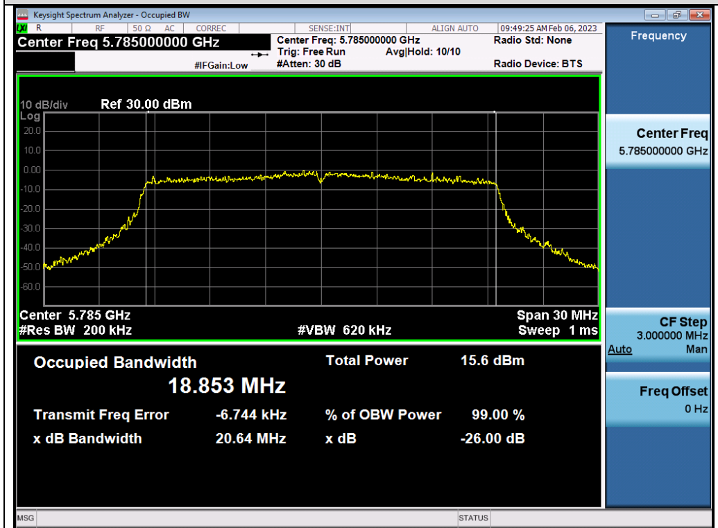
Test_Graph_802.11ax20_ANT2_5785_MCS0_OBW
