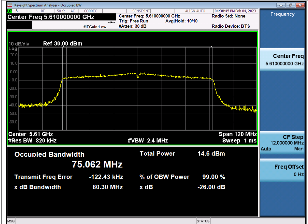
Test_Graph_802.11ac80_ANT2_5610_MCS9_OBW
