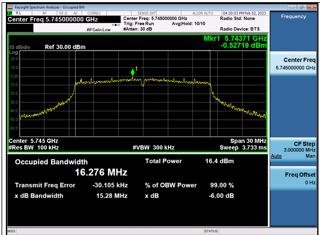
Test_Graph_802.11a_ANT1_5745_6Mbps_DTSBW
