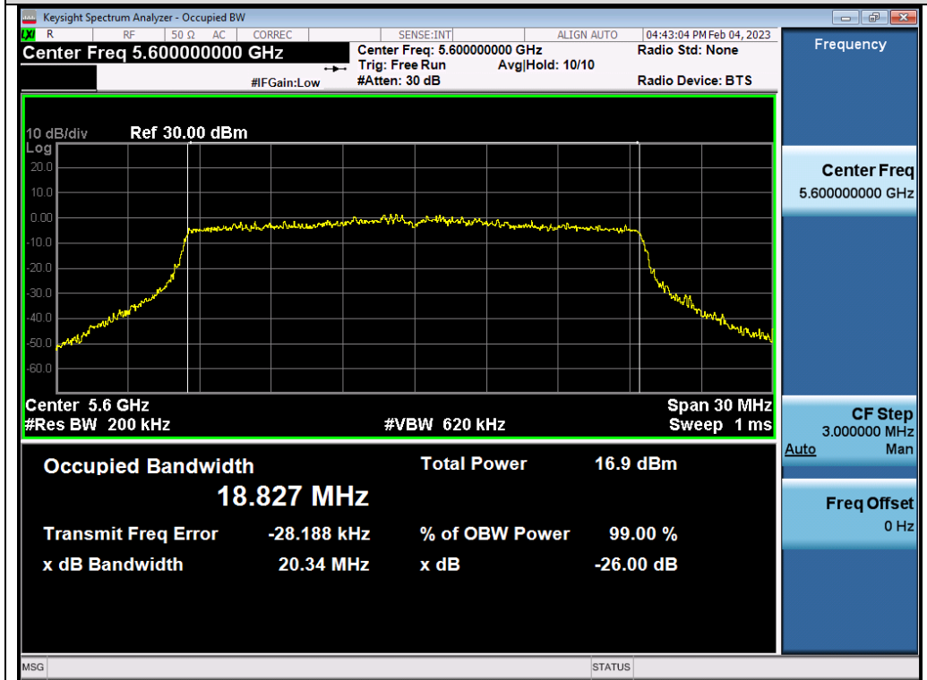
Test_Graph_802.11ax20_ANT2_5600_MCS0_OBW
