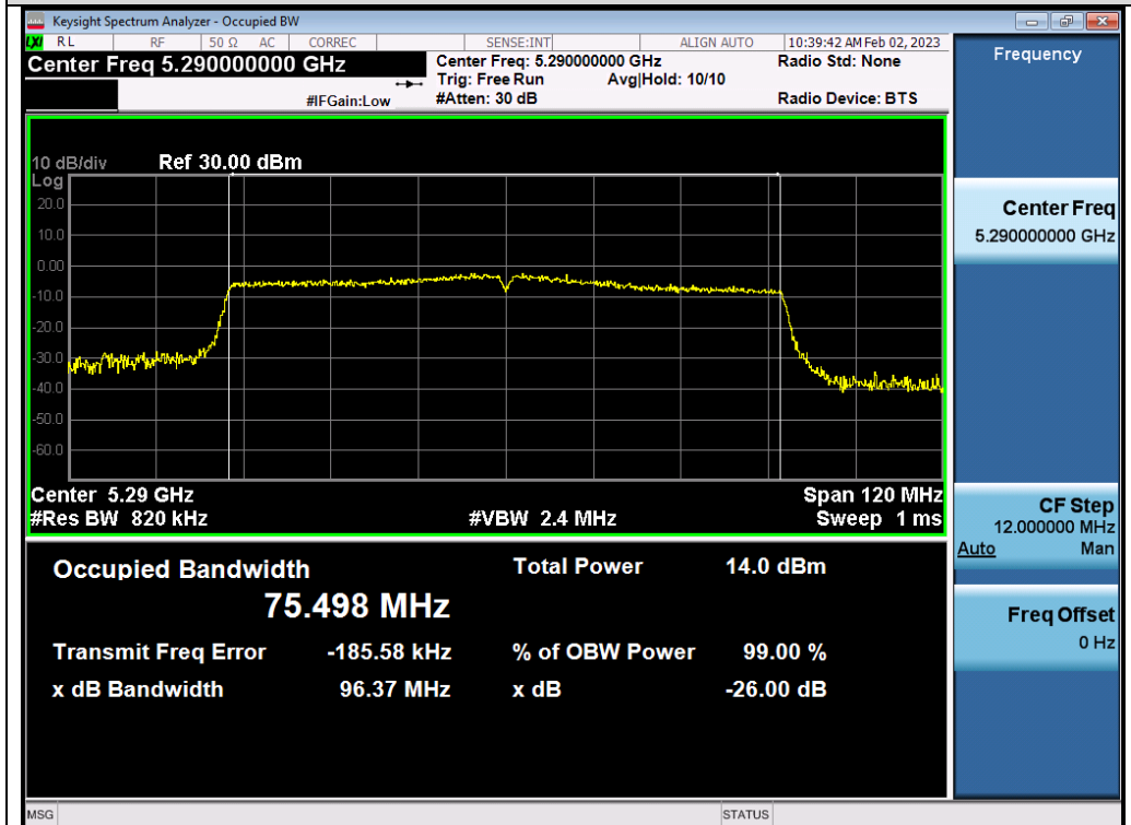
Test_Graph_802.11ac80_ANT1_5290_MCS9_OBW
