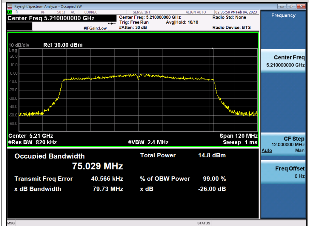
Test_Graph_802.11ac80_ANT2_5210_MCS9_OBW
