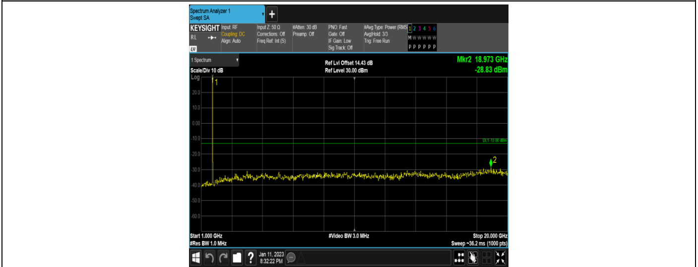
Band4-3MHz-16QAM-19965-1RB#0-Range2:1000~20000MHz
