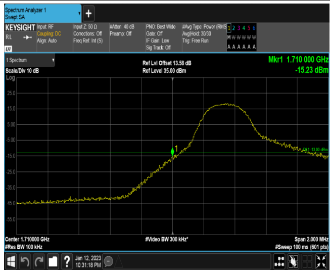
Band4-5MHz-QPSK-19975-1RB#0
