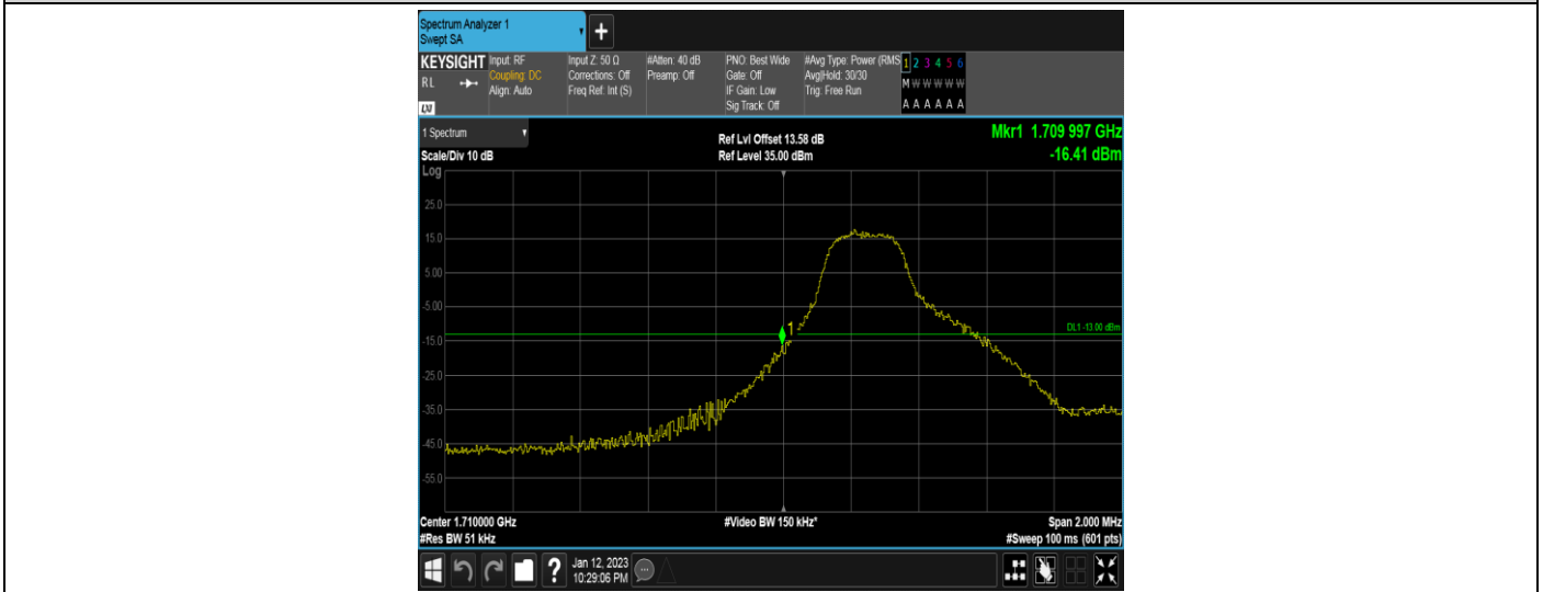
Band4-3MHz-16QAM-19965-1RB#14
