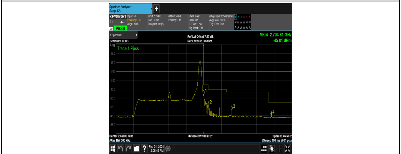
Band41-15MHz-QPSK-41515-1RB#74
