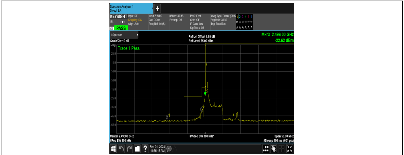
Band41-5MHz-16QAM-39675-1RB#24
