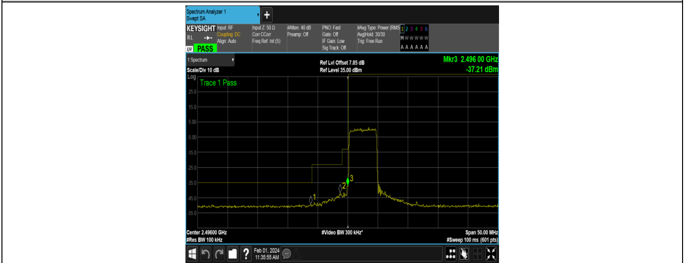
Band41-5MHz-16QAM-39675-25RB#0
