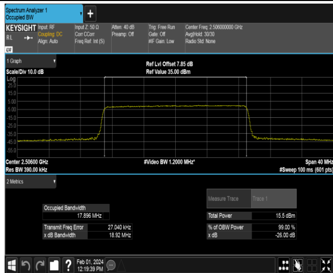
Band41-20MHz-16QAM-40620-100RB#0
