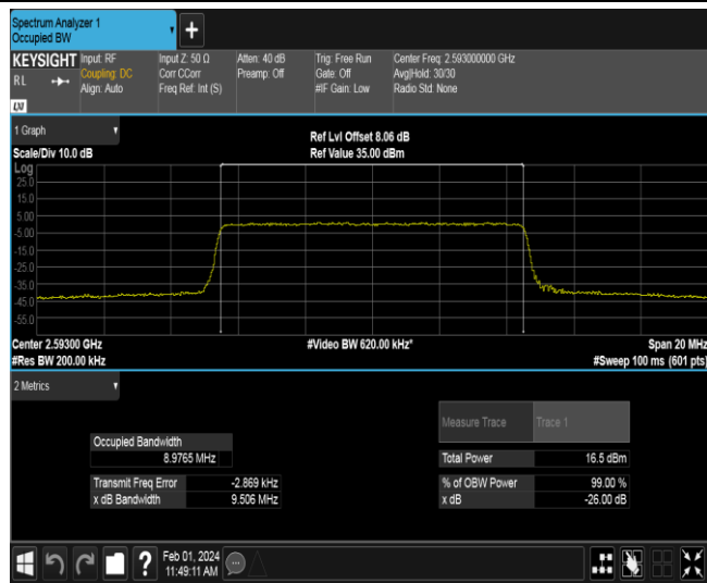
Band41-10MHz-16QAM-41540-50RB#0
