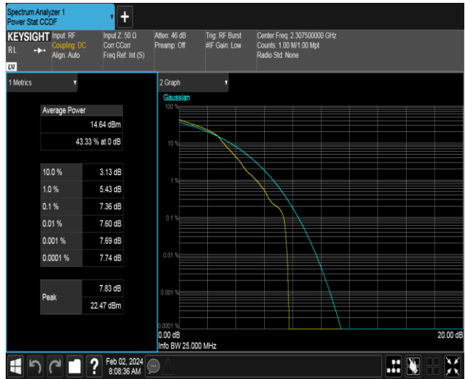
Band40-5MHz-16QAM-38725-25RB#0
