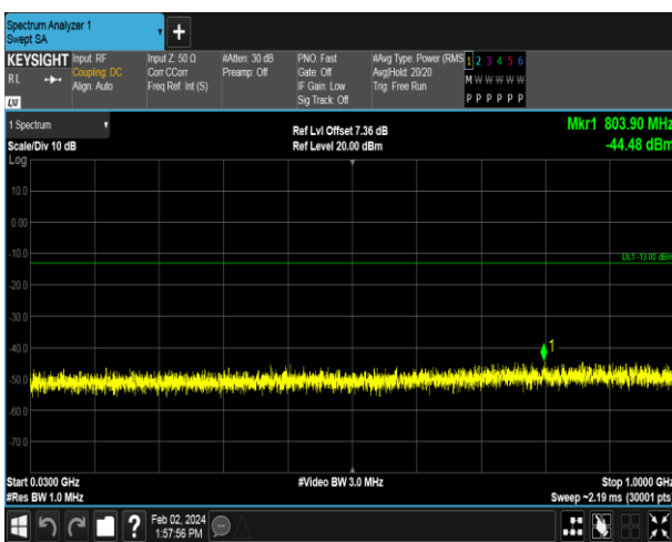
WCDMA 1700_RMC 12.2kps_MCH
