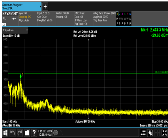
WCDMA 1900_RMC 12.2kps_MCH
