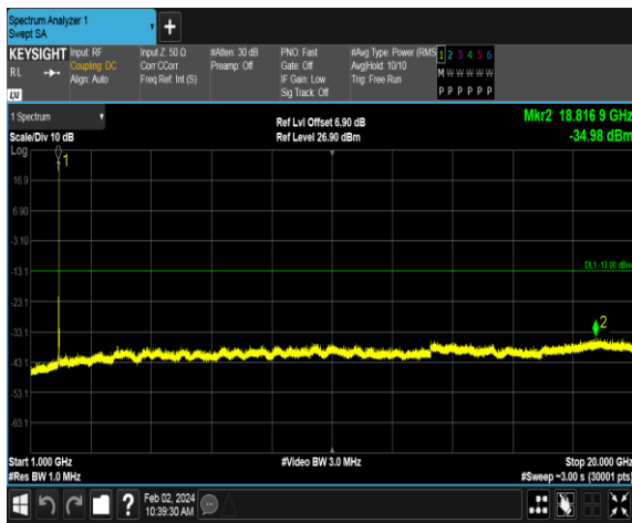
WCDMA 1900_RMC 12.2kps_HCH
