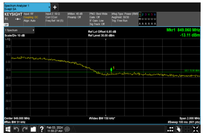
WCDMA850_HSUPA_ Highest Channel
