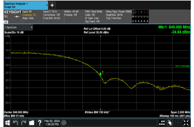
WCDMA850_HSDPA_ Highest Channel
