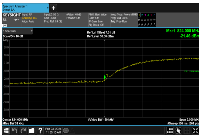
WCDMA850_HSUPA_ Lowest Channel
