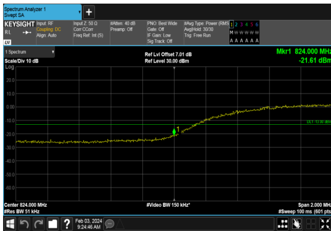
WCDMA850_HSUPA_ Lowest Channel
