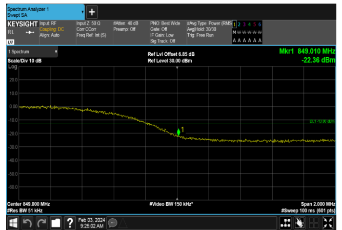
WCDMA850_HSUPA_ Highest Channel
