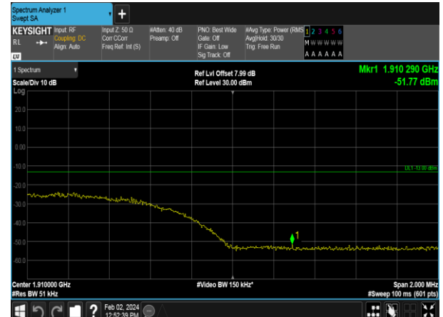
WCDMA1900_HSUPA_ Highest Channel
