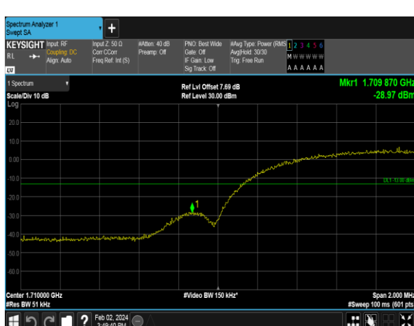
WCDMA1700_HSUPA_ Lowest Channel
