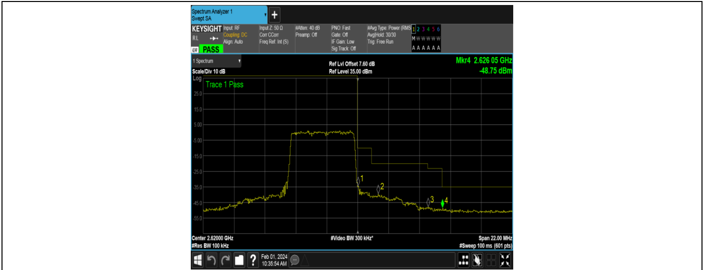
Band38-10MHz-QPSK-37800-1RB#0
