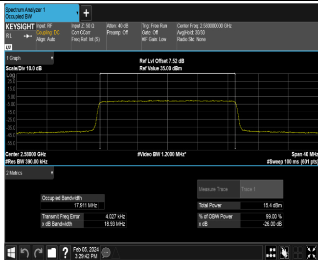
Band38-20MHz-16QAM-38000-100RB#0
