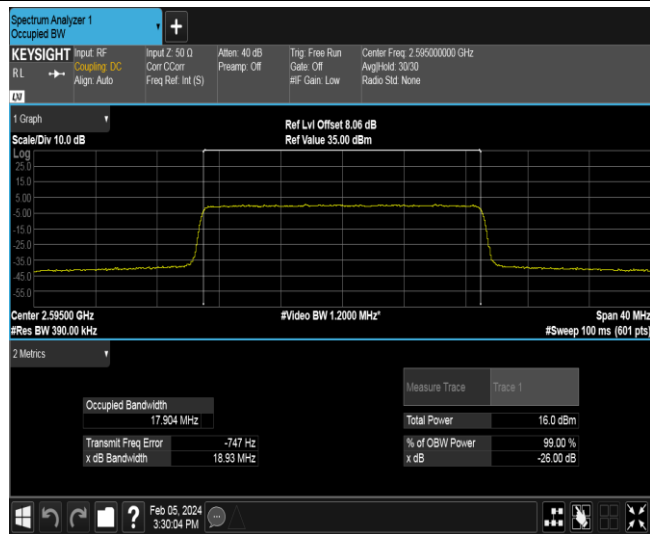
Band38-20MHz-16QAM-38000-100RB#0
