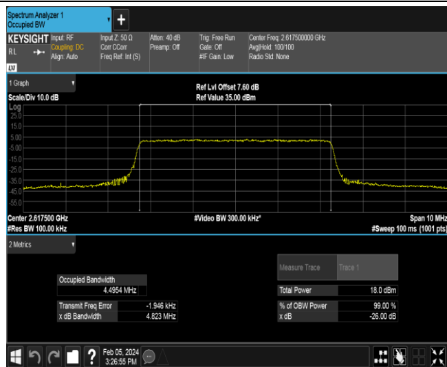
Band38-5MHz-QPSK-38225-25RB#0
