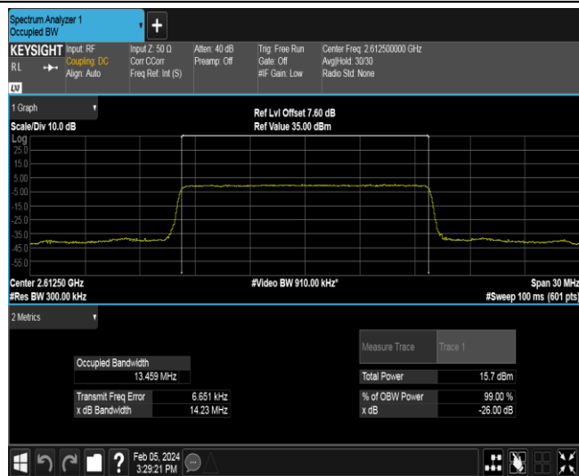
Band38-15MHz-16QAM-38175-75RB#0
