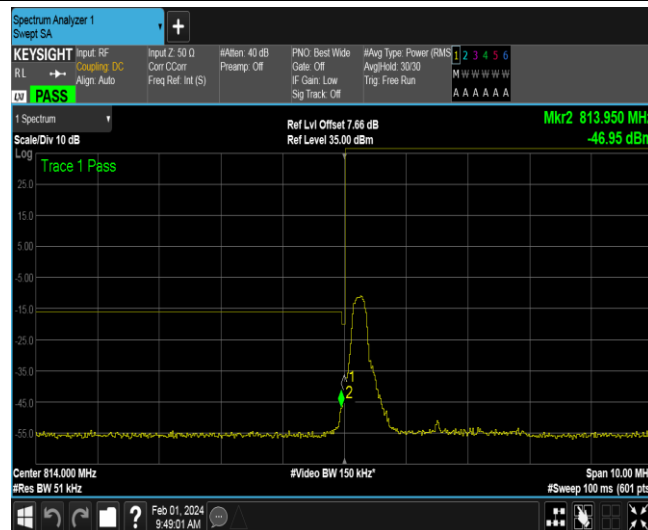
Band26-3MHz-QPSK-26705-1RB#14
