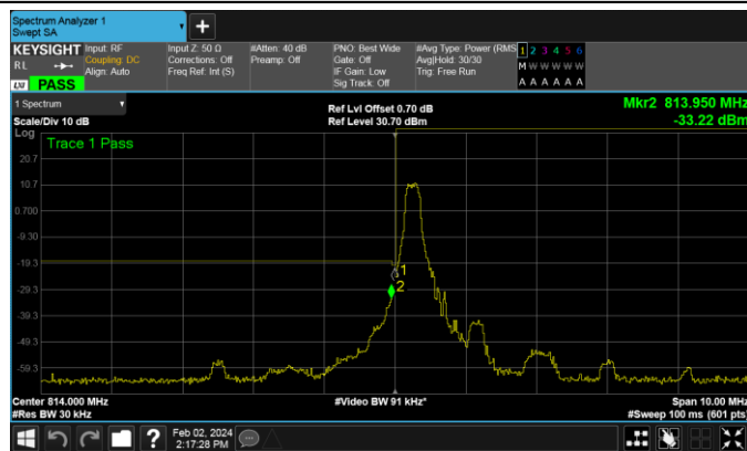
Band26-1.4MHz-16QAM-26697-1RB#5
