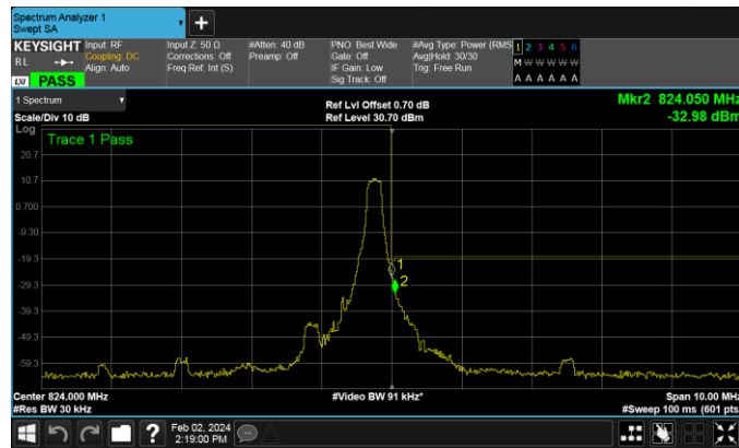
Band26-1.4MHz-16QAM-26783-6RB#0
