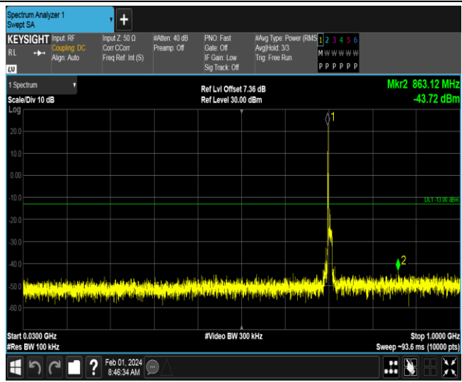
Band17-10MHz-16QAM-23800-1RB#0-Range1:30~1000MHz
