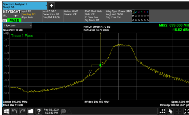
Band12-3MHz-16QAM-23025-1RB#14
