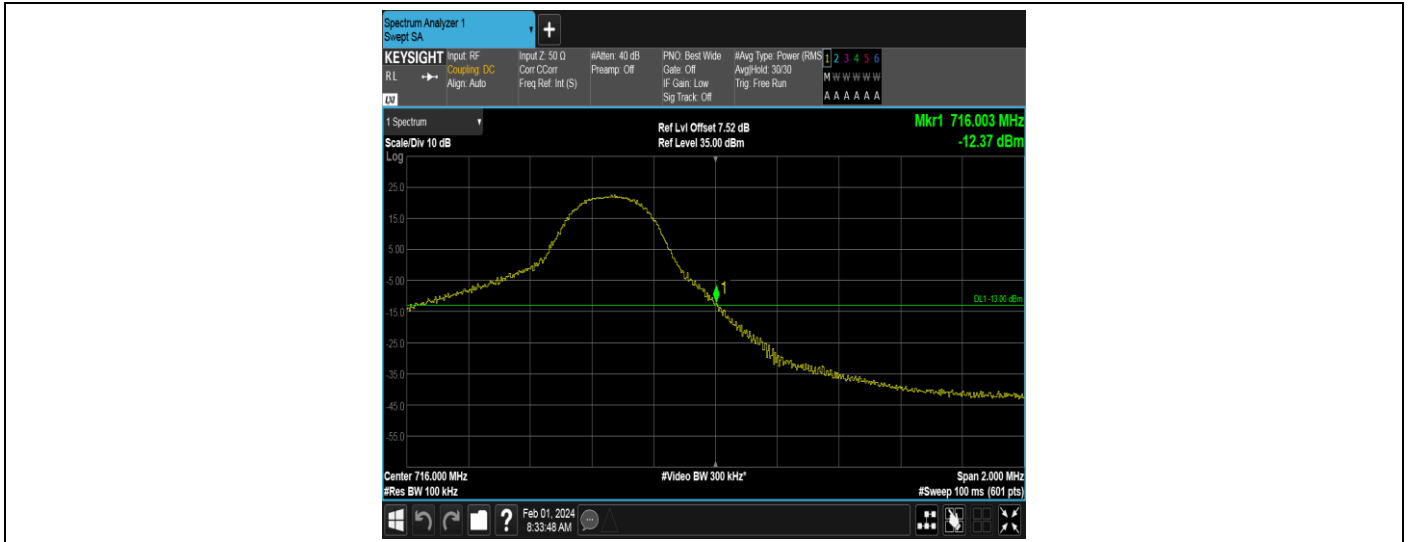
Band12-5MHz-QPSK-23155-25RB#0
