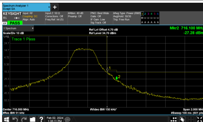
Band12-3MHz-16QAM-23165-15RB#0
