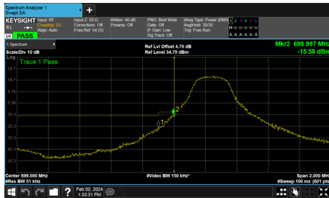
Band12-3MHz-QPSK-23025-1RB#14
