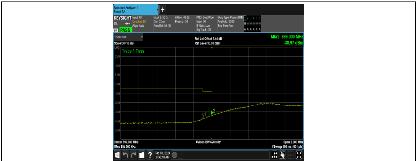
Band12-10MHz-16QAM-23060-50RB#0
