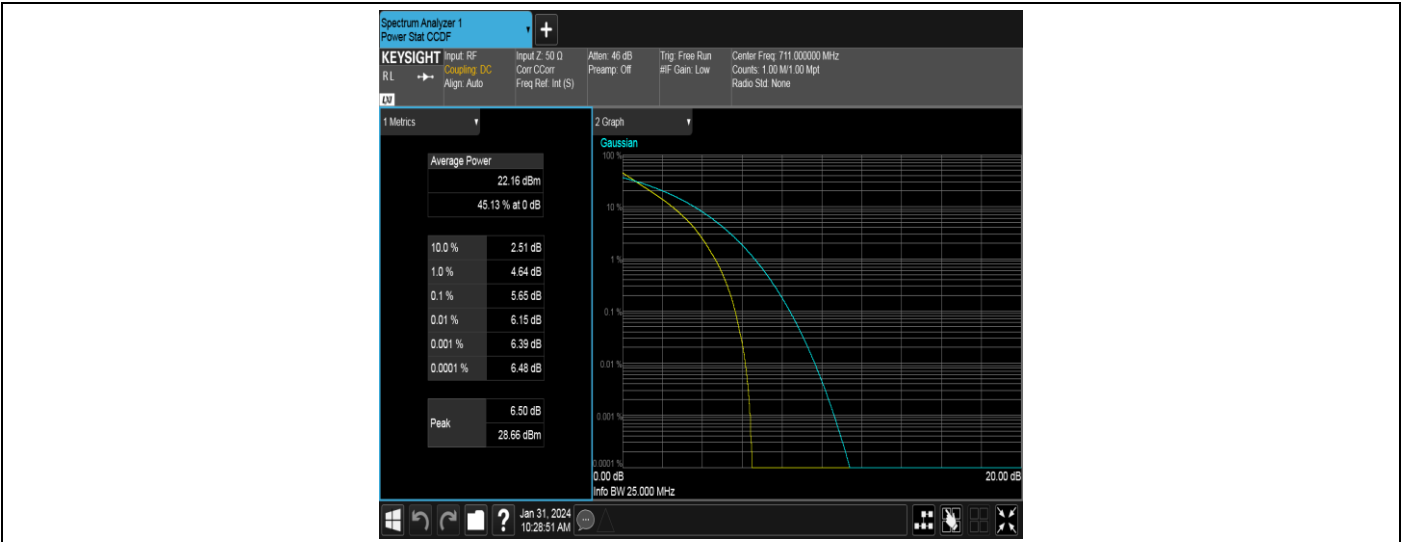
Band12-10MHz-16QAM-23060-1RB#0
