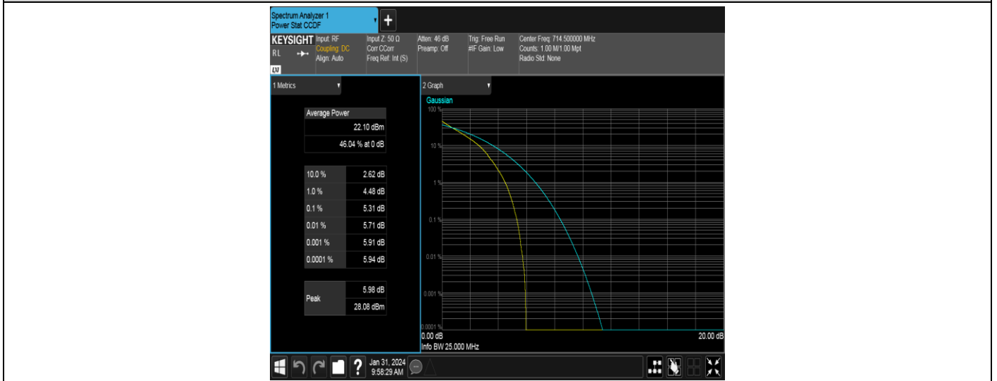
Band12-3MHz-16QAM-23025-1RB#0
