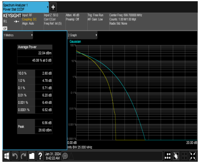
Band12-1.4MHz-QPSK-23095-1RB#0
