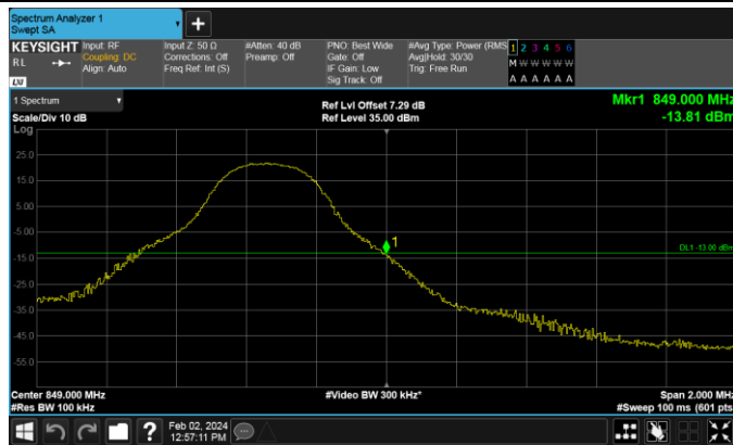
Band5-5MHz-QPSK-20625-25RB#0
