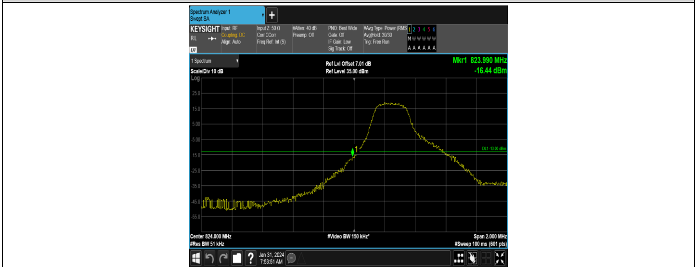
Band5-3MHz-QPSK-20415-1RB#14
