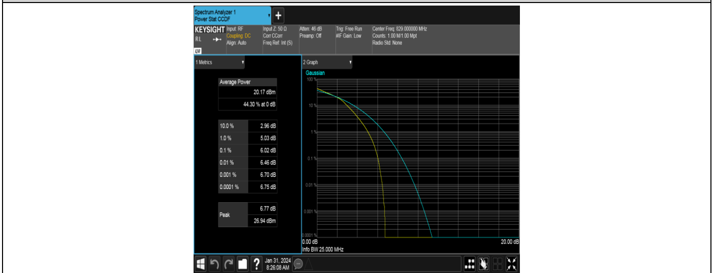
Band5-10MHz-16QAM-20525-1RB#0
