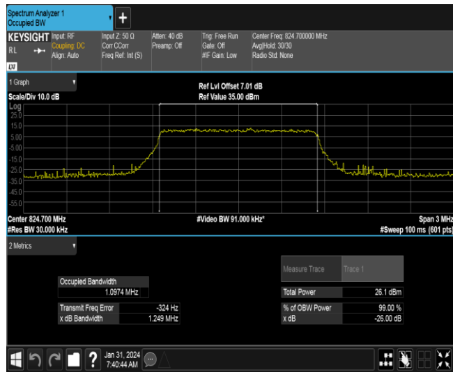
Band5-1.4MHz-QPSK-20525-6RB#0
