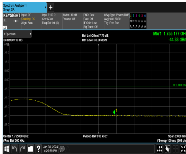
Band4-15MHz-QPSK-20325-1RB#74
