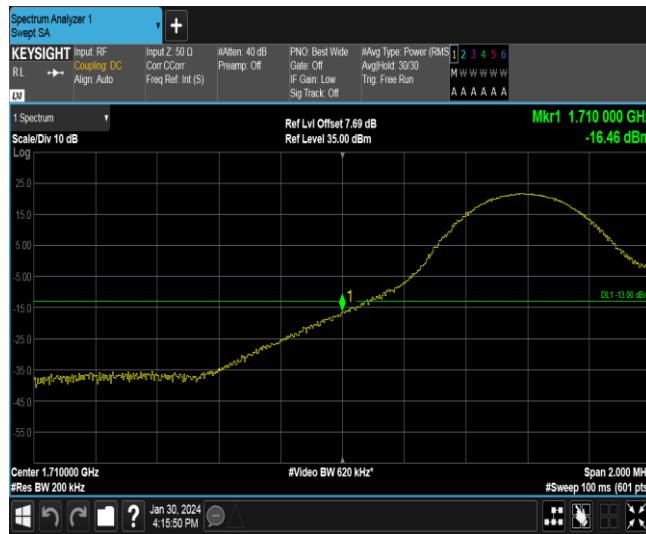
Band4-10MHz-QPSK-20000-1RB#49
