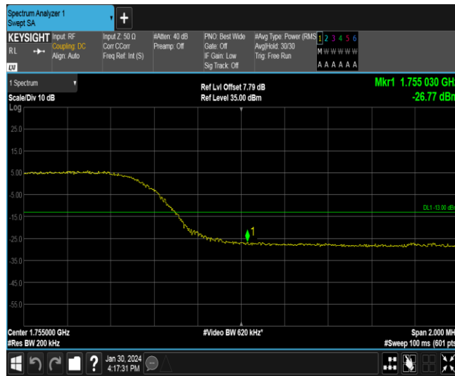
Band4-10MHz-16QAM-20000-1RB#0
