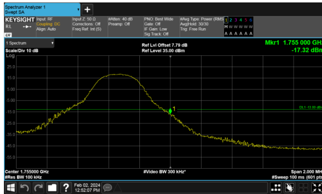
Band4-5MHz-QPSK-20375-25RB#0
