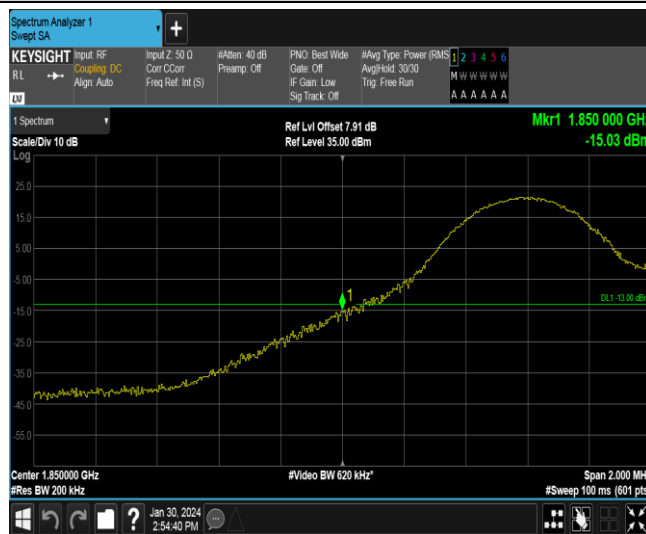
Band2-10MHz-16QAM-18650-1RB#0
