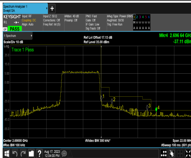
Band41-5MHz-16QAM-41565-25RB#0
