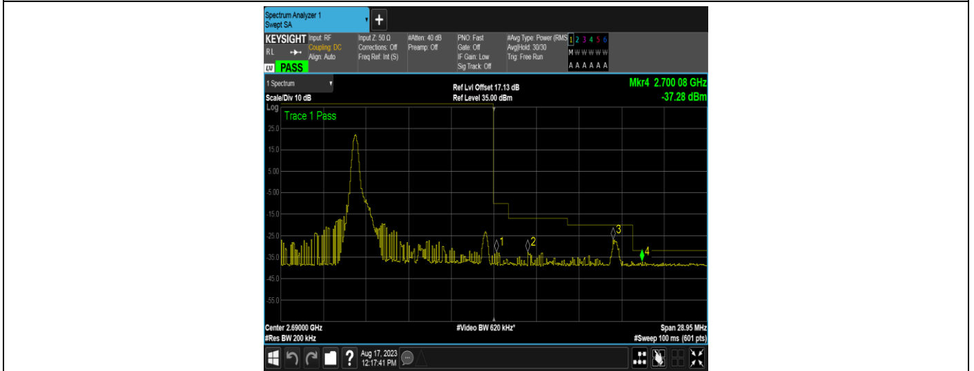
Band41-10MHz-16QAM-41540-1RB#0
