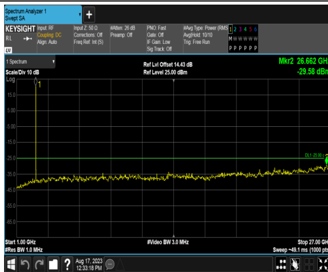
Band41-15MHz-16QAM-40620-1RB#0-Range2:1000~27000MHz
