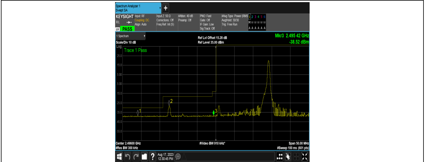
Band41-15MHz-QPSK-39725-75RB#0
