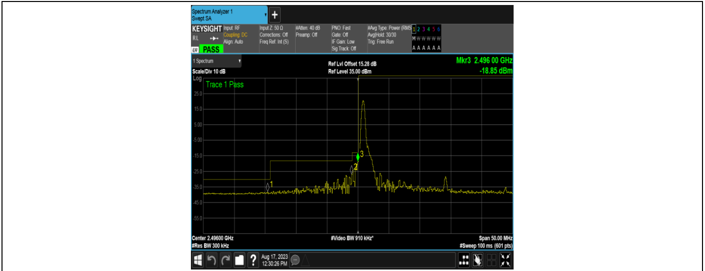
Band41-15MHz-QPSK-39725-1RB#74
