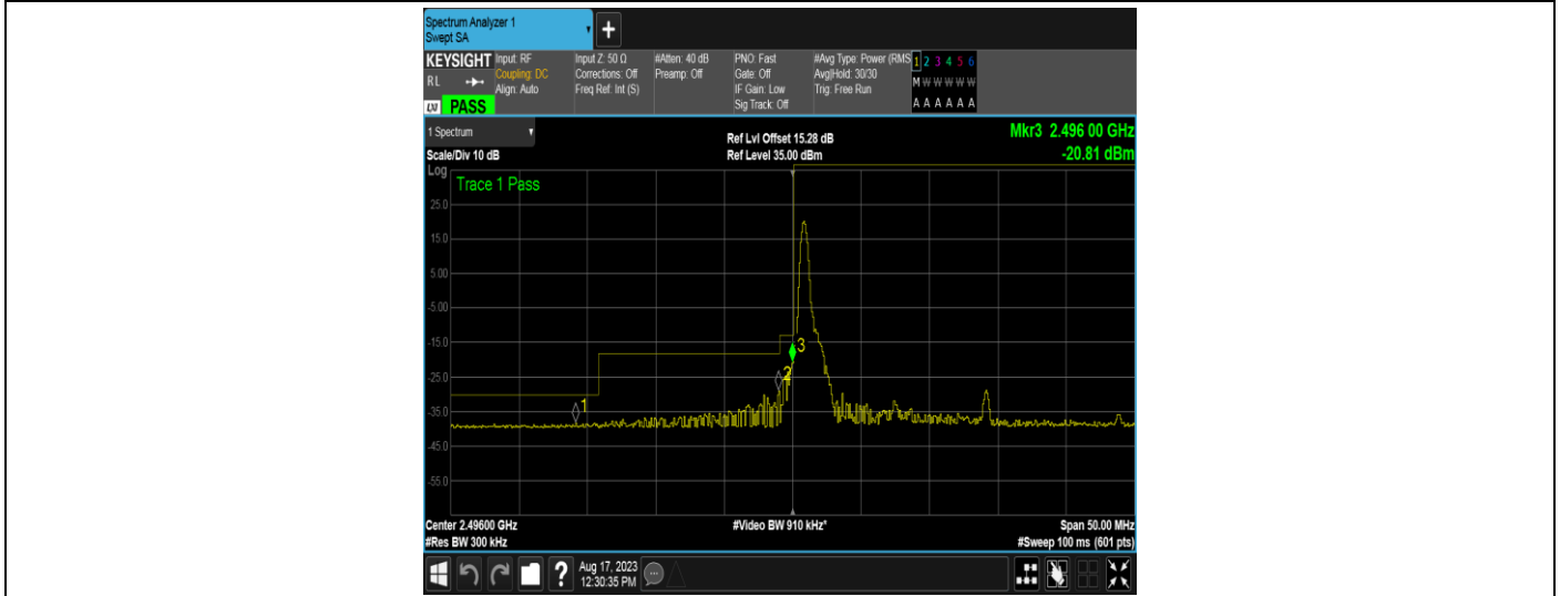
Band41-15MHz-16QAM-39725-1RB#74
