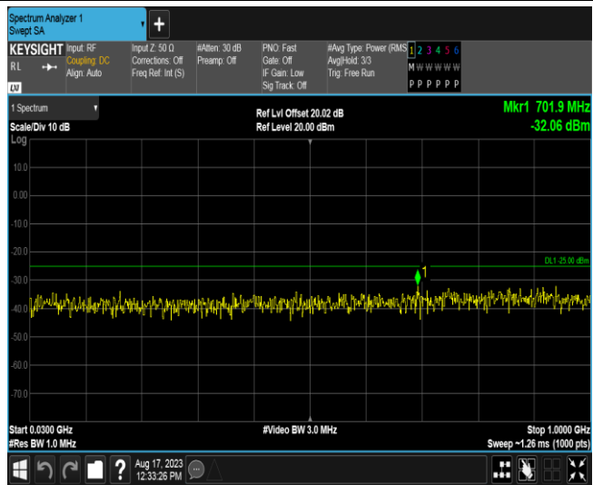
Band41-15MHz-QPSK-41515-1RB#0-Range1:30~1000MHz
