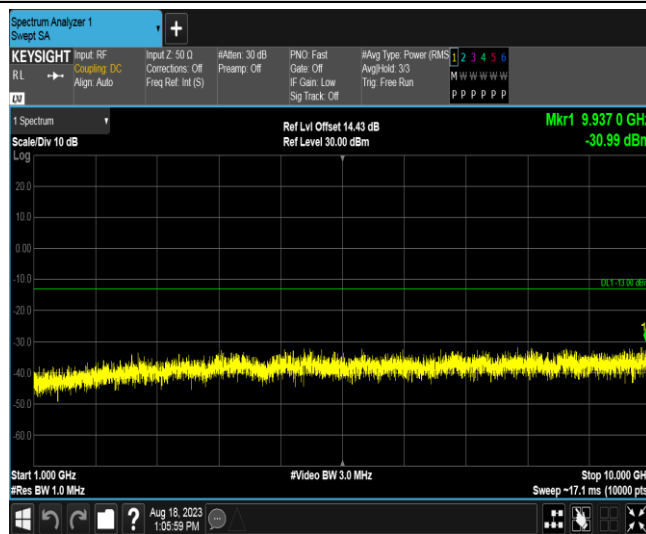
Band26-5MHz-16QAM-26715-1RB#0-Range2:1000~10000MHz
