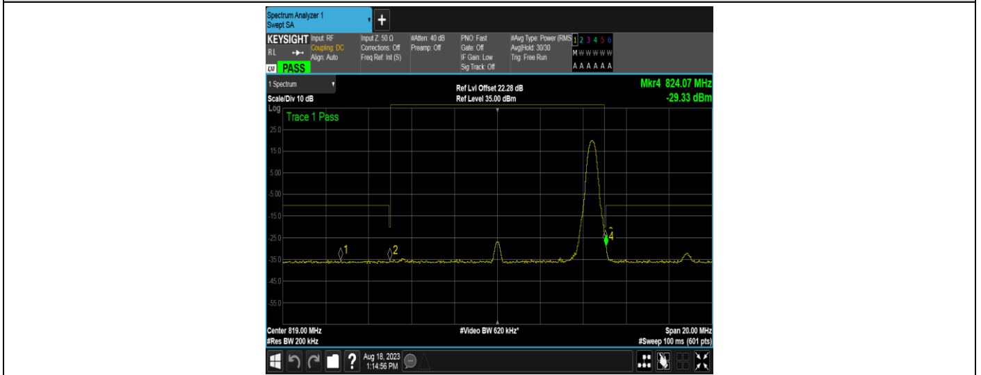
Band26-10MHz-QPSK-26740-50RB#0
