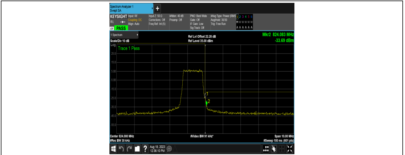
Band26-3MHz-QPSK-26705-1RB#0
