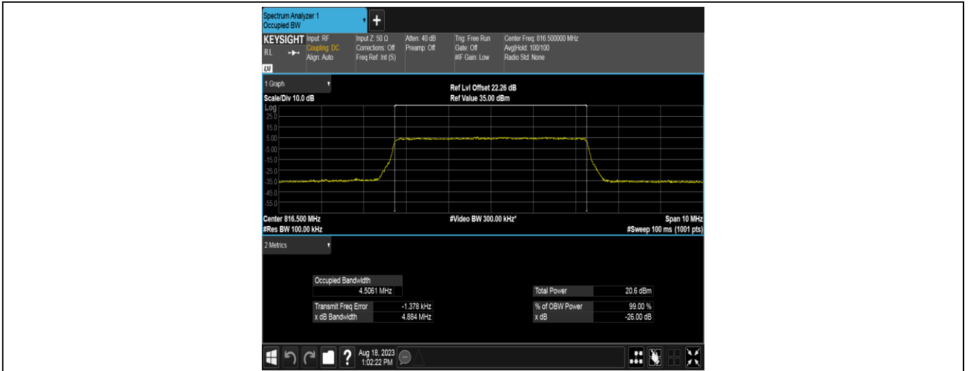
Band26-5MHz-16QAM-26740-25RB#0
