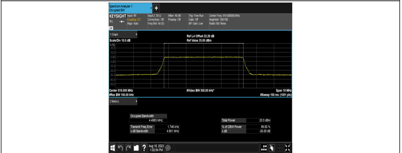
Band26-5MHz-16QAM-26765-25RB#0
