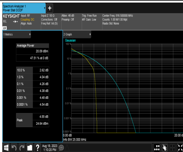
Band26-5MHz-QPSK-26715-1RB#0
