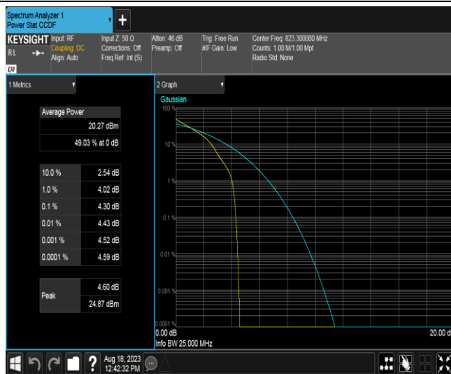
Band26-1.4MHz-QPSK-26783-1RB#0
