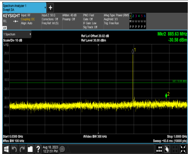
Band12-10MHz-QPSK-23095-1RB#0-Range1:30~1000MHz
