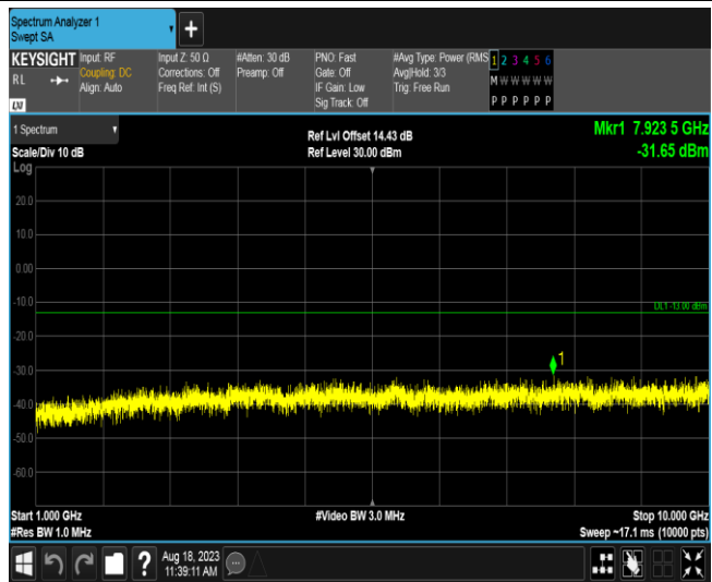
Band12-1.4MHz-QPSK-23095-1RB#0-Range2:1000~10000MHz
