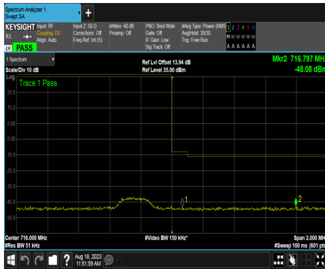
Band12-3MHz-16QAM-23165-1RB#14
