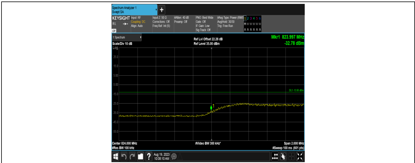
Band5-5MHz-16QAM-20425-25RB#0
