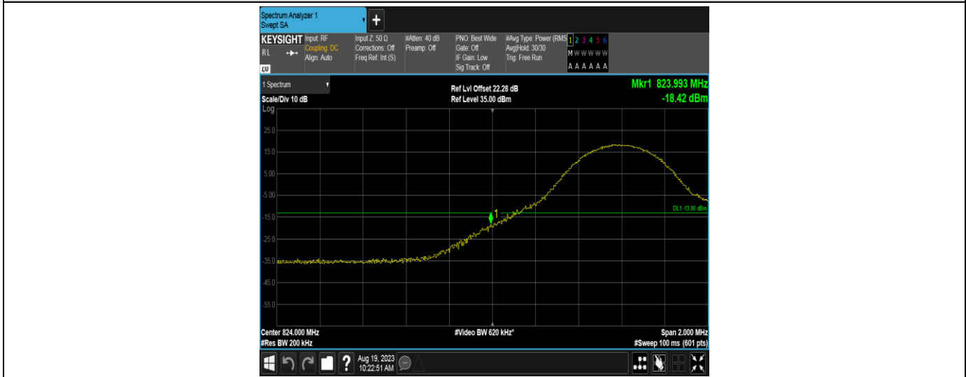
Band5-10MHz-16QAM-20450-1RB#49
