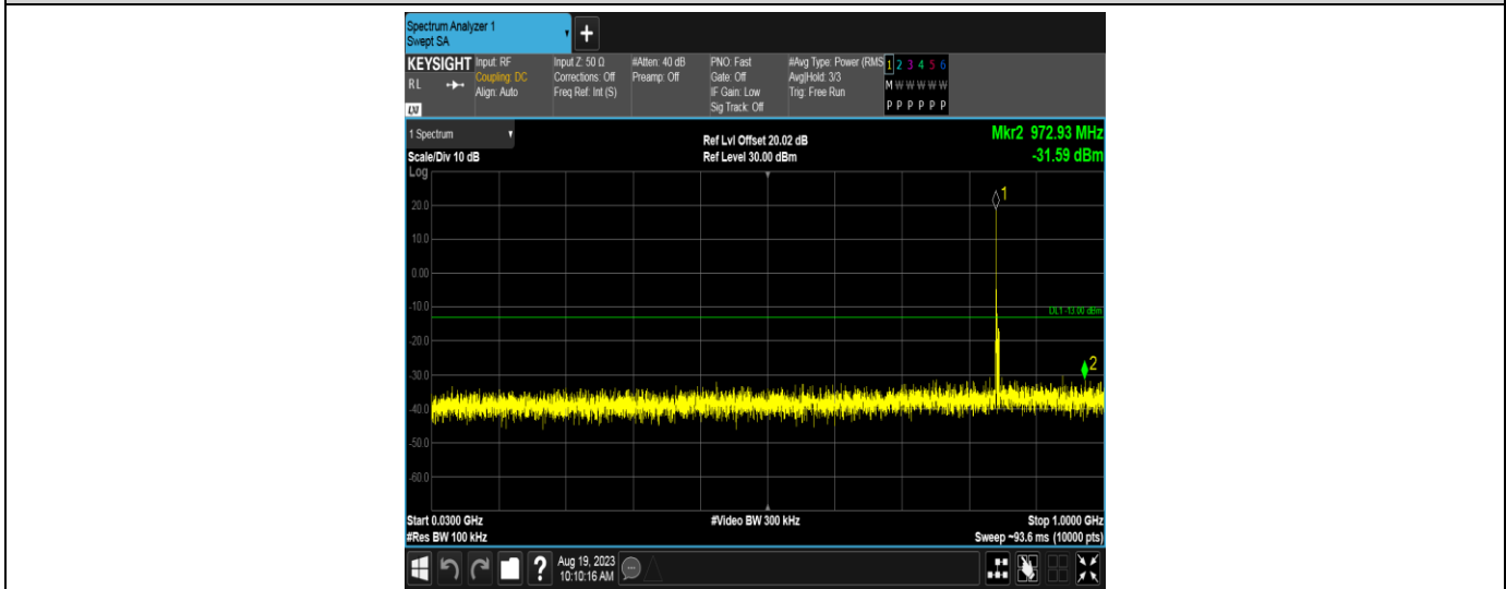
Band5-5MHz-QPSK-20625-1RB#0-Range1:30~1000MHz
