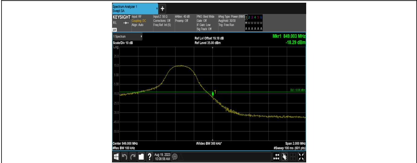
Band5-5MHz-QPSK-20625-1RB#24
