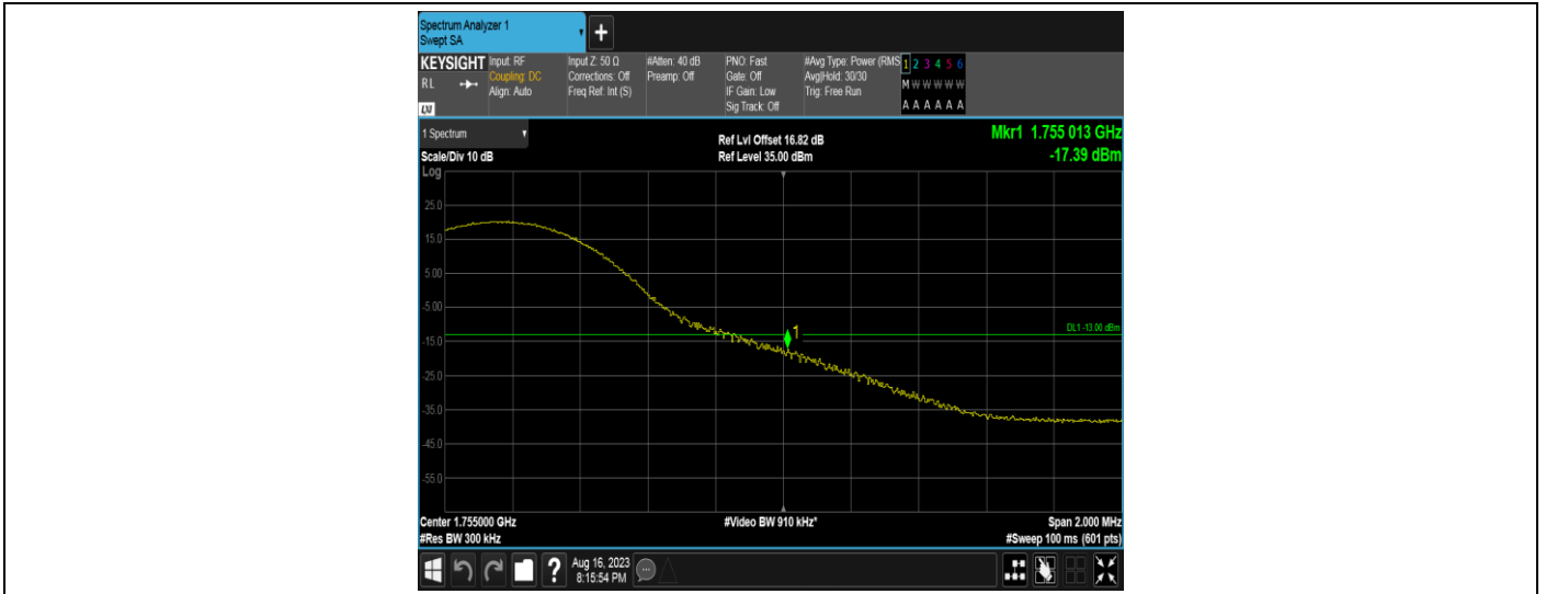
Band4-15MHz-QPSK-20325-75RB#0
