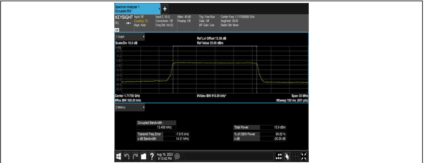
Band4-15MHz-16QAM-20175-75RB#0
